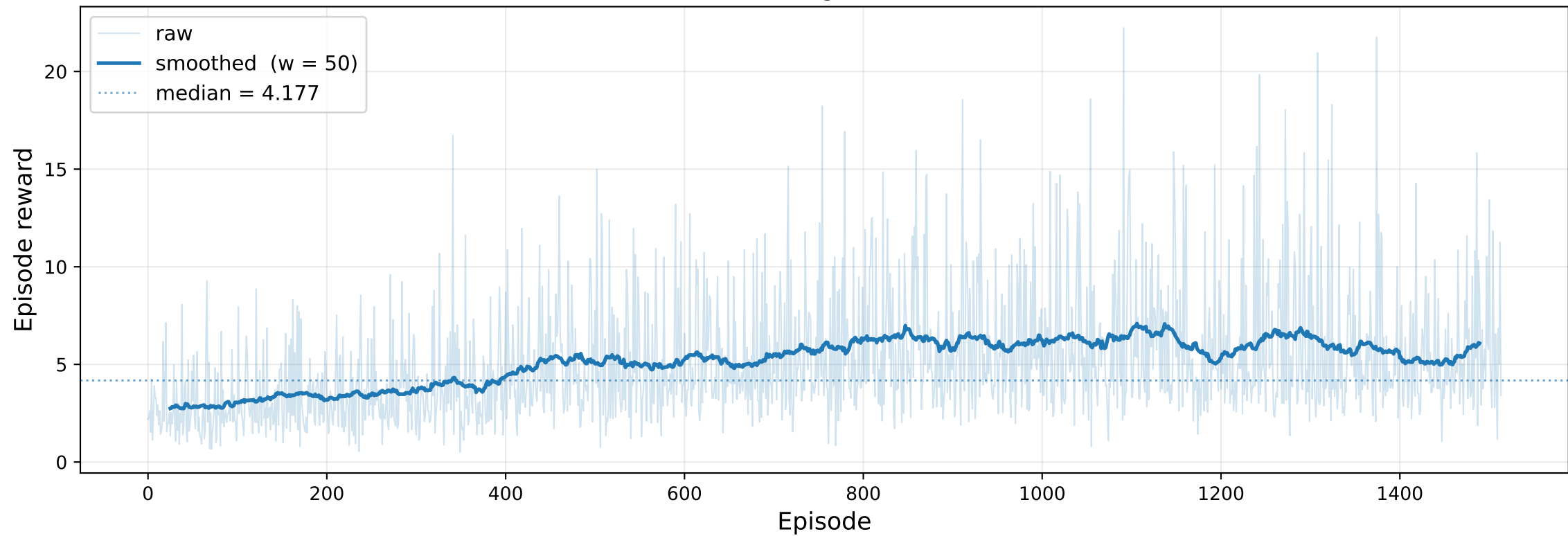
MDPO - Training reward (total)
