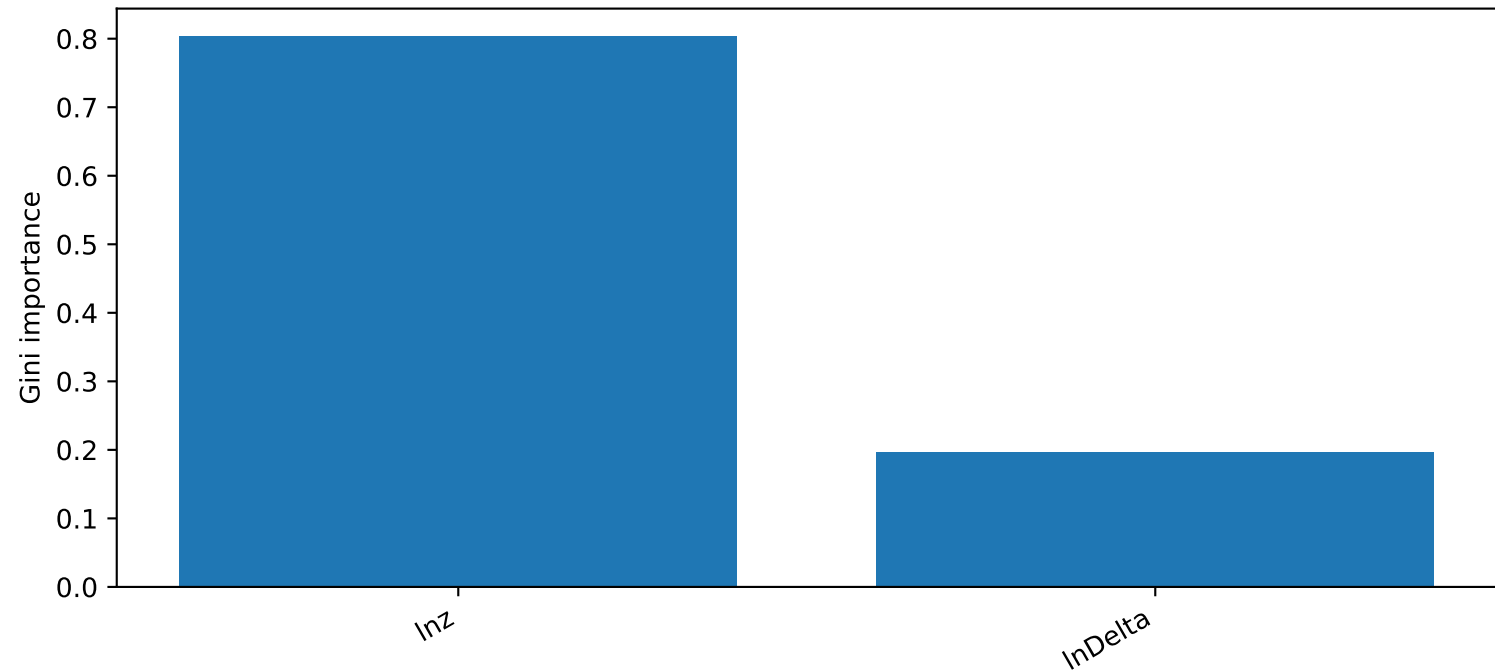
Surrogate DT - Feature Importance for Grooming Decisions
