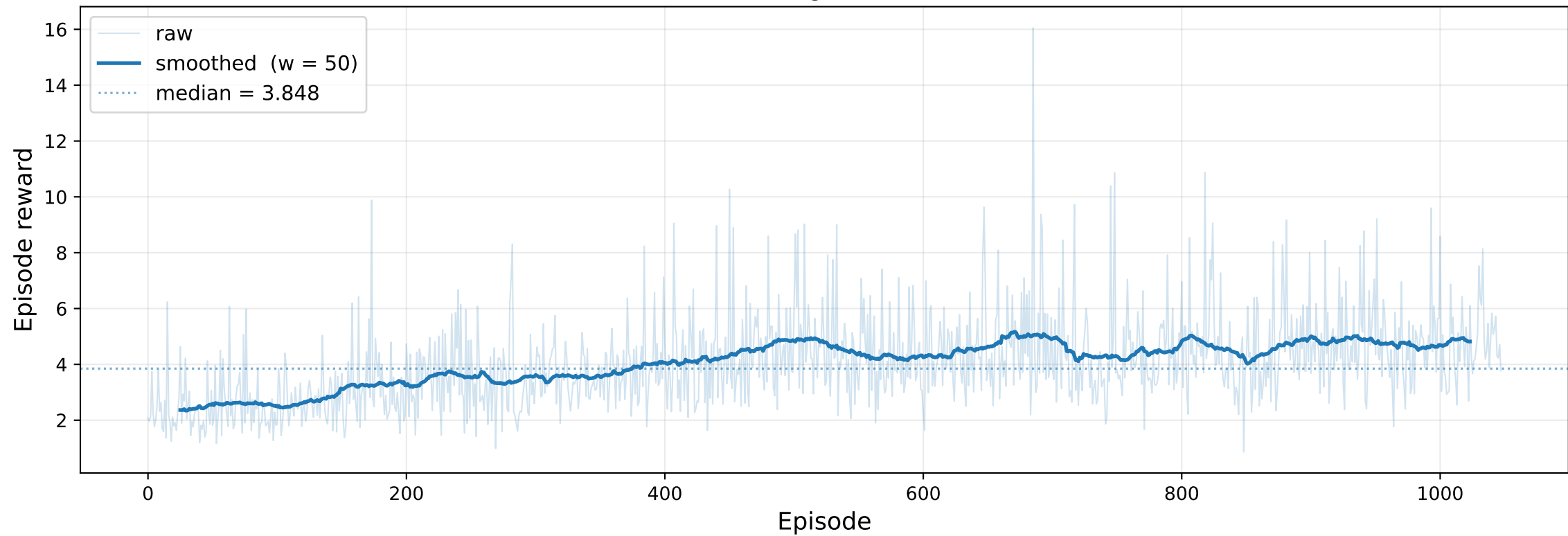
PPO - Training reward (total)
