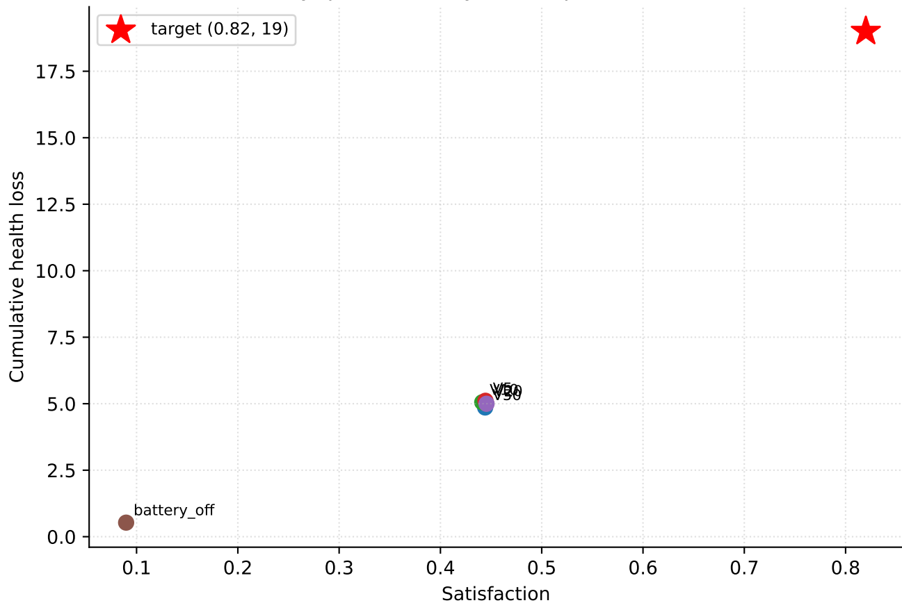
assist = LyapunovGreedy V-sweep (satisfaction vs HL)
