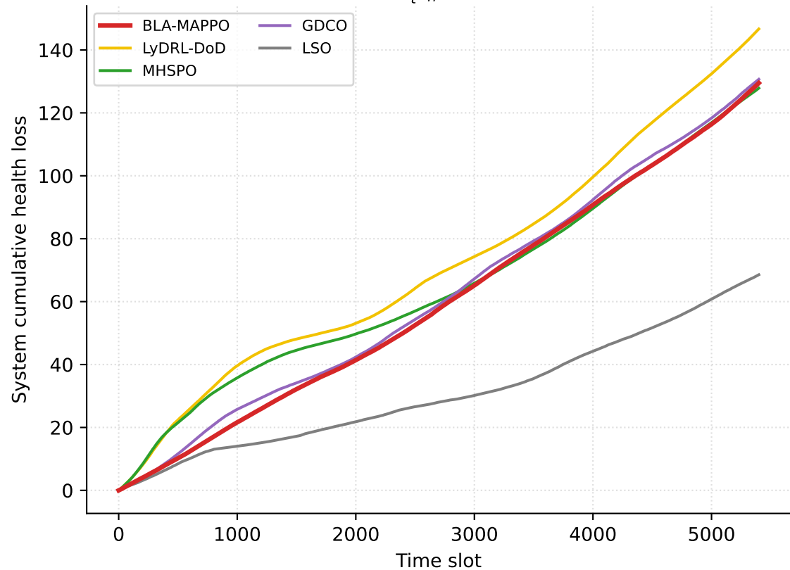
Secant (proposed): \sum_t \sum_n [\mathcal{L}(DoD_{with}) - \mathcal{L}(DoD_{wo})]
