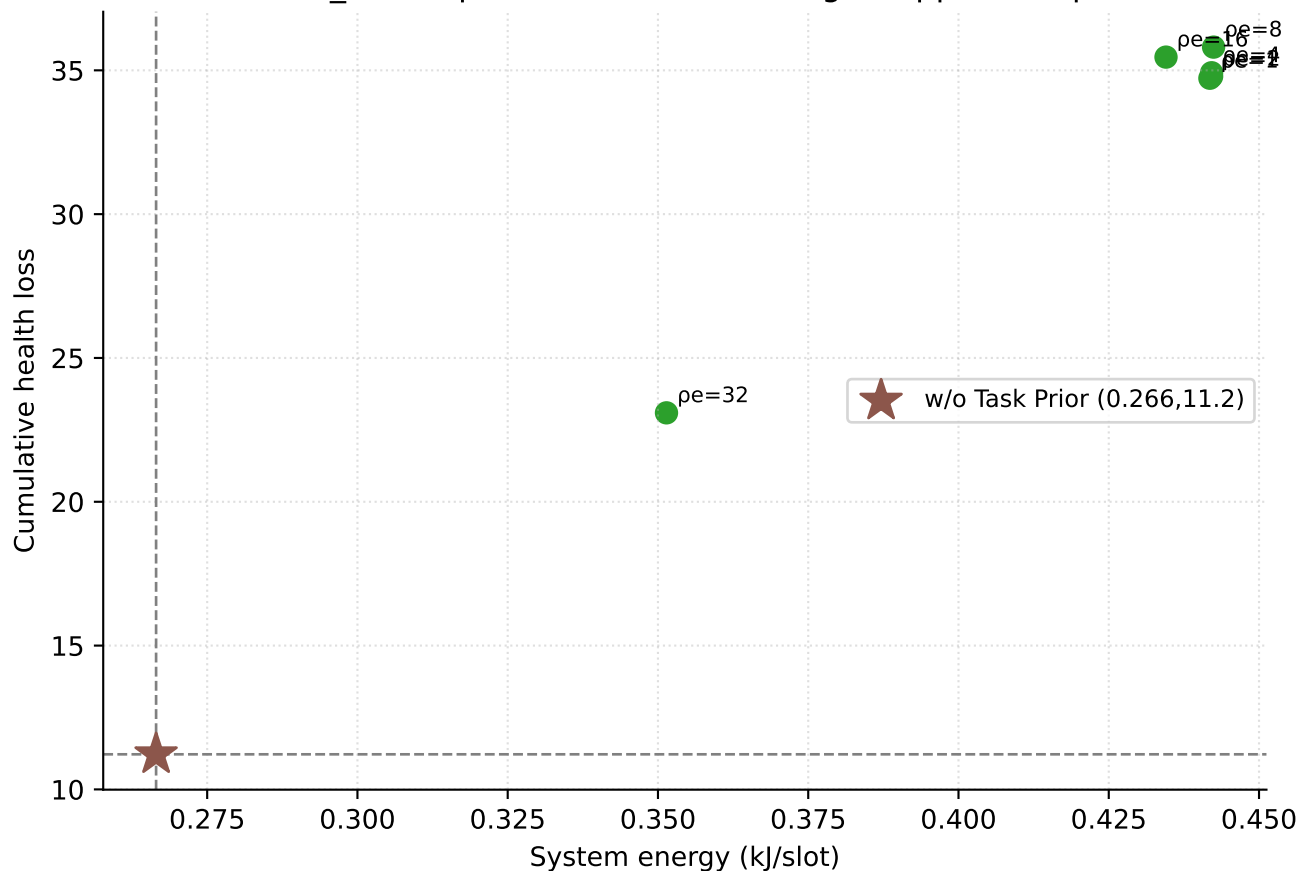
MHSPO rho_e sweep vs w/o Task Prior (target: upper-left quadrant)
