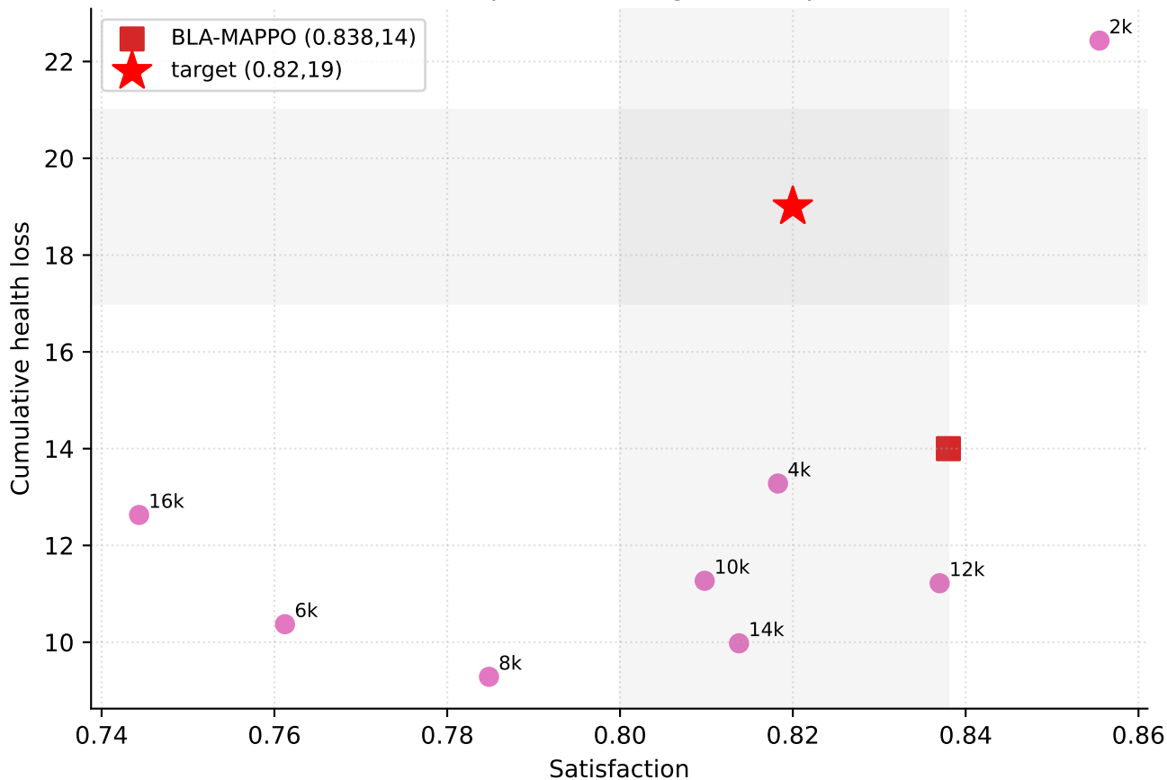
w/o Task Prior checkpoints vs target (new params, 1 seed)
