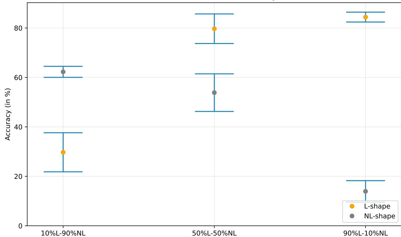
Dual Source - L vs NL Accuracy
