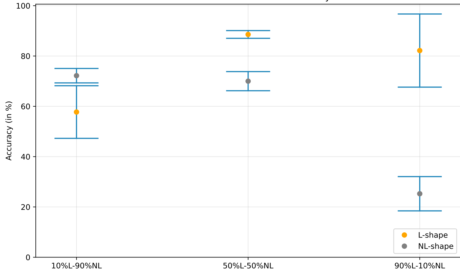
Feature Invariant - L vs NL Accuracy
