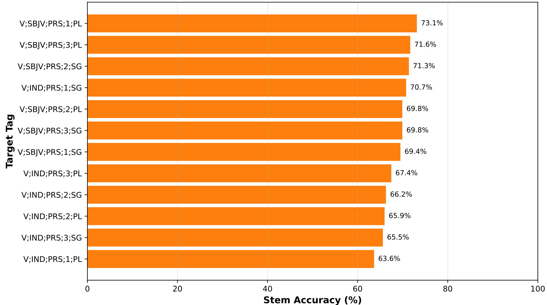
Stem Accuracy by Target Tag - 50%L-50%NL - Character Separated
