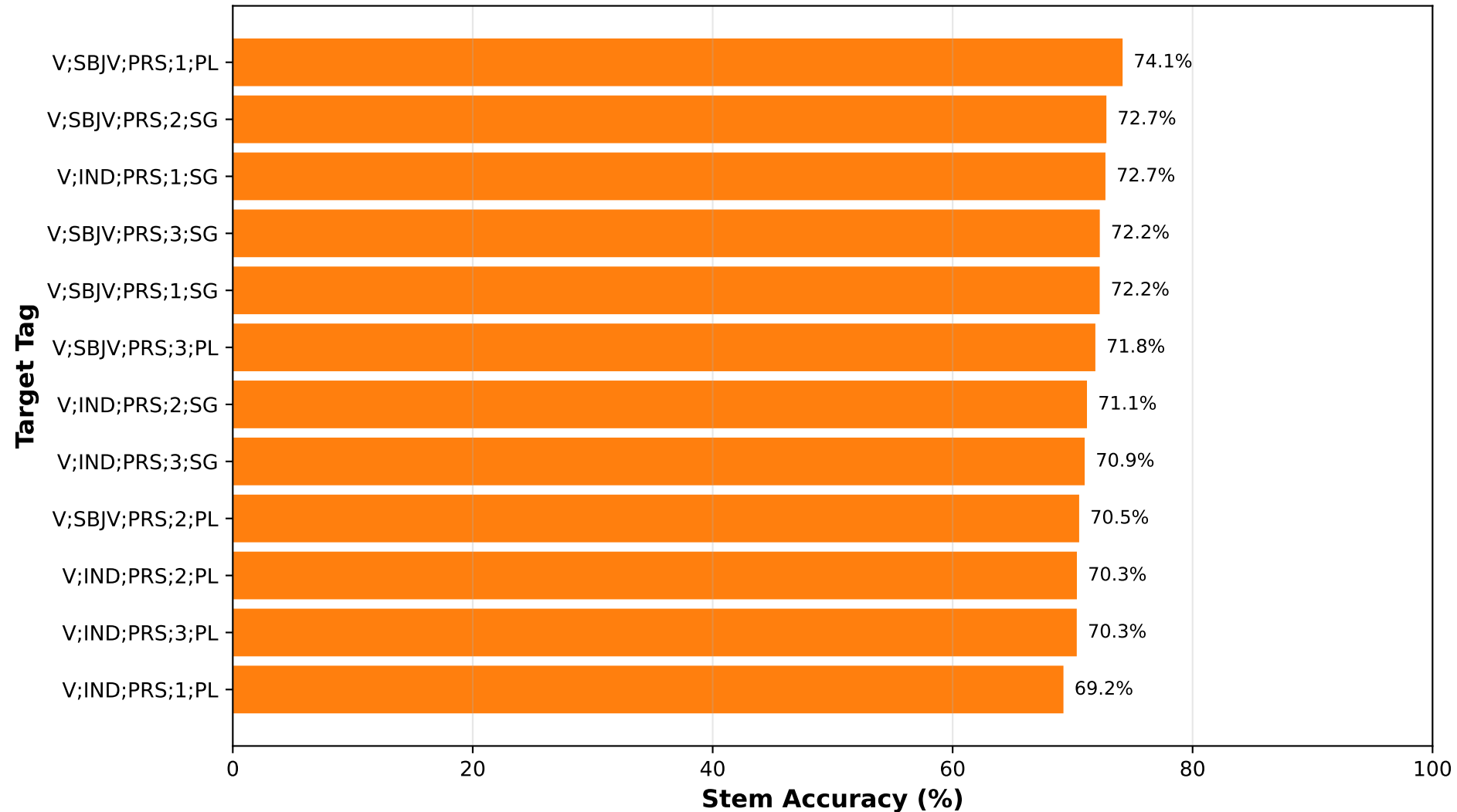
Stem Accuracy by Target Tag - Character Separated
