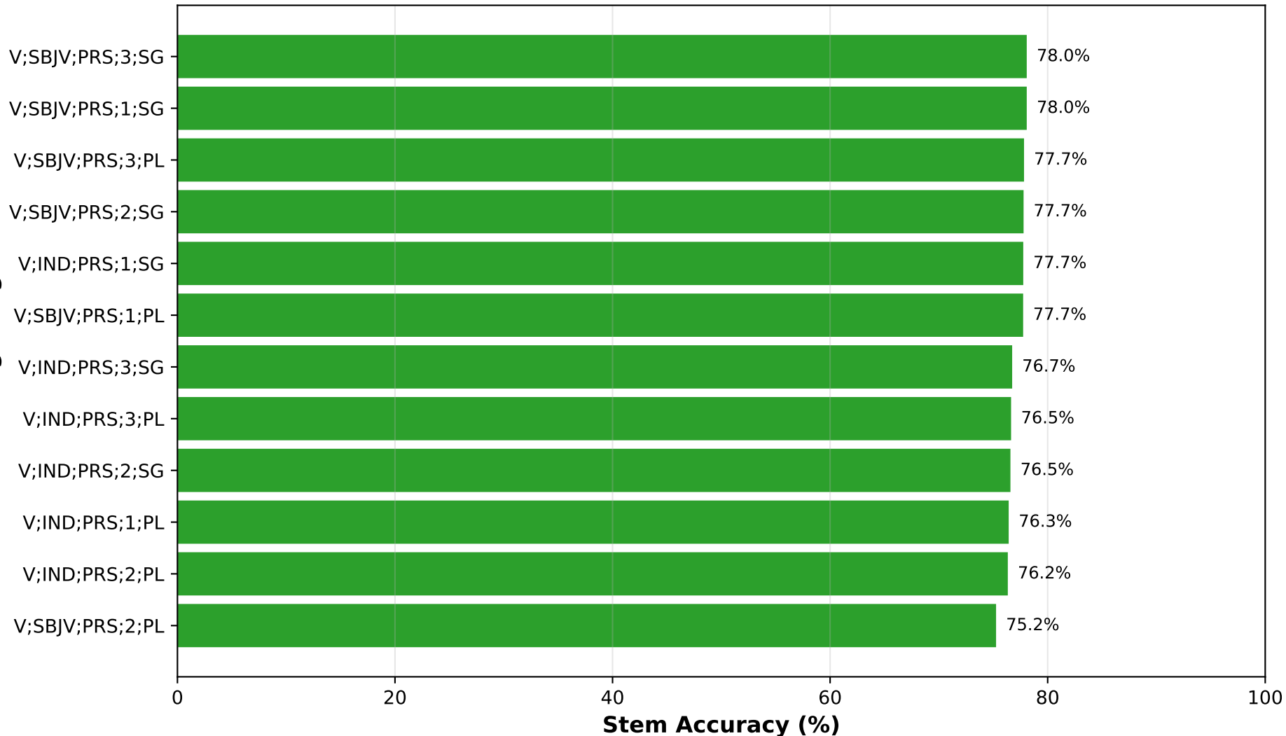
Stem Accuracy by Target Tag - 10%L-90%NL - Feature Invariant
