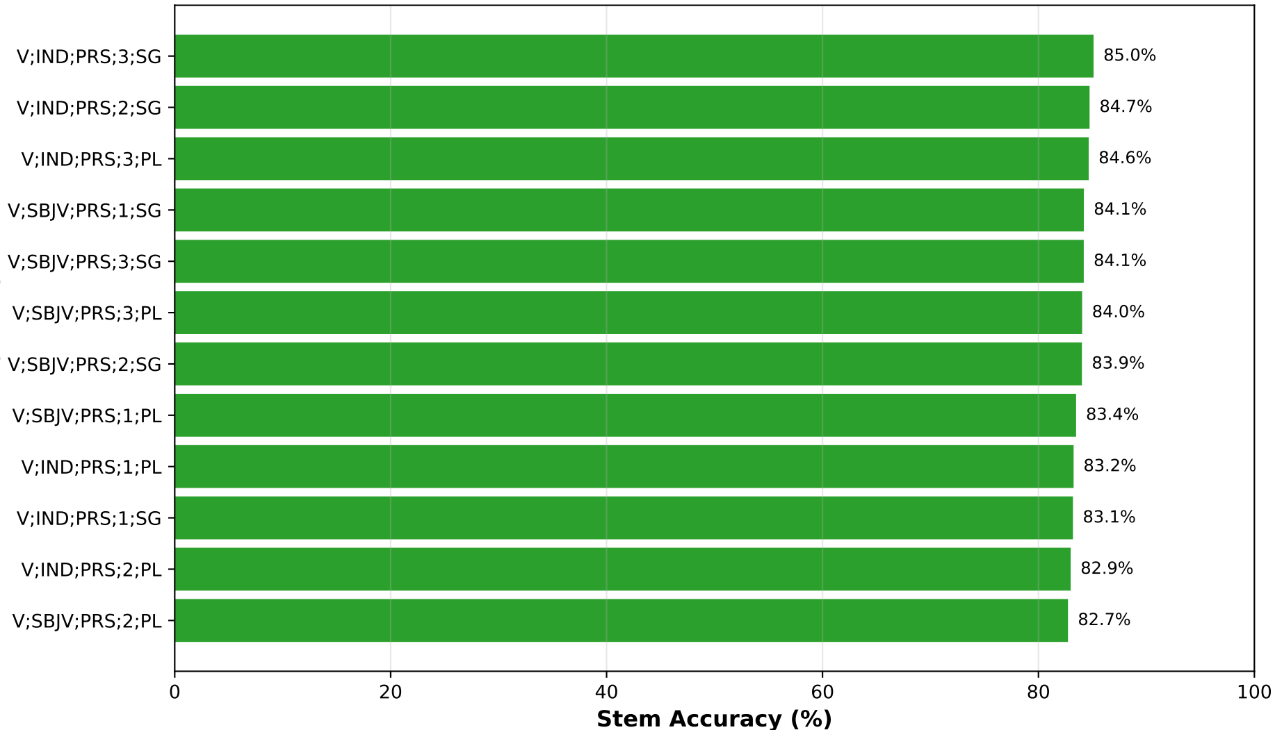
Stem Accuracy by Target Tag - 50%L-50%NL - Feature Invariant
