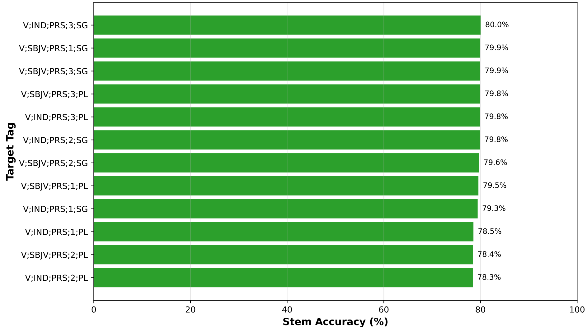
Stem Accuracy by Target Tag - Feature Invariant
