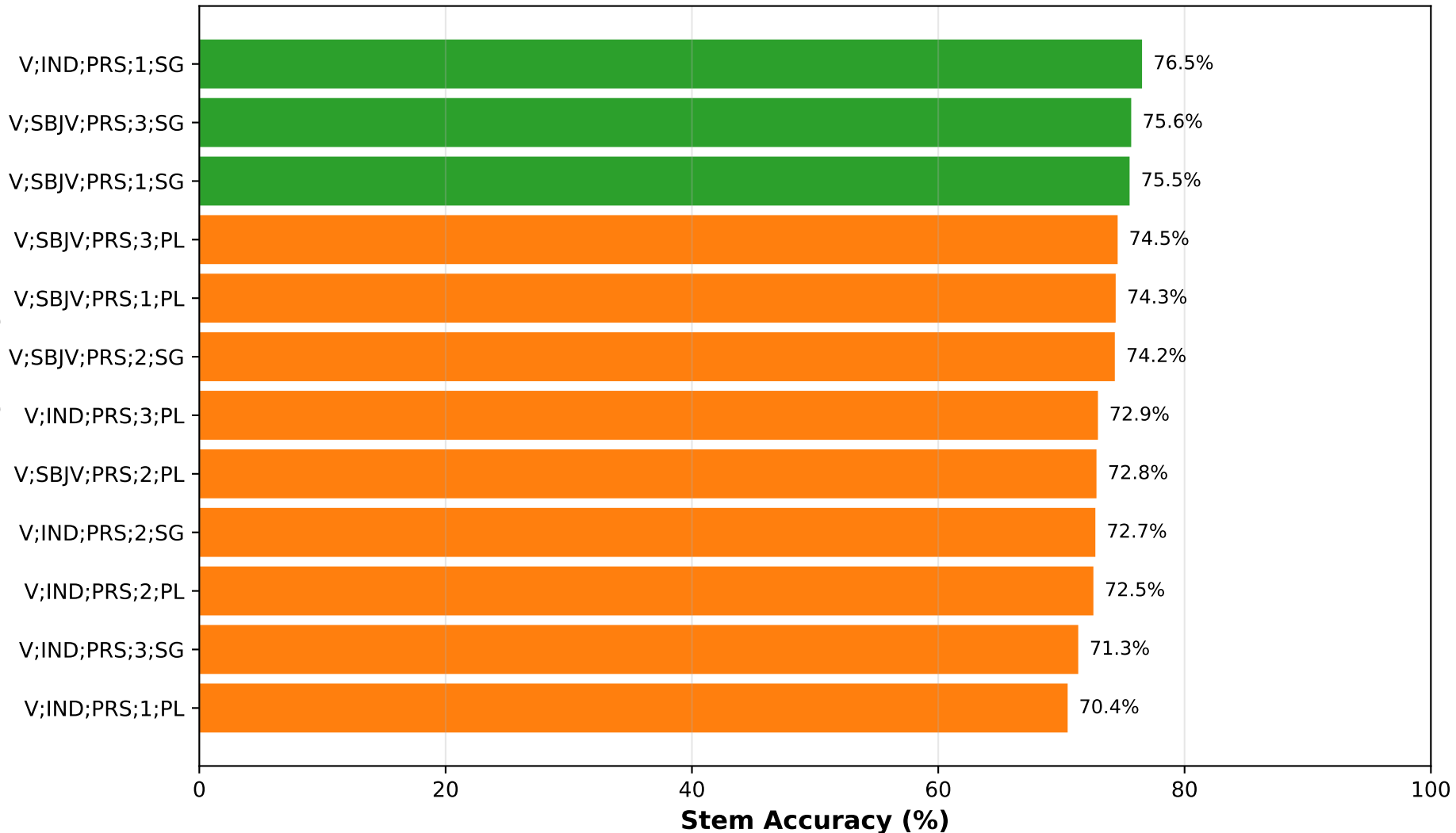
Stem Accuracy by Target Tag - 50%L-50%NL - Vanilla
