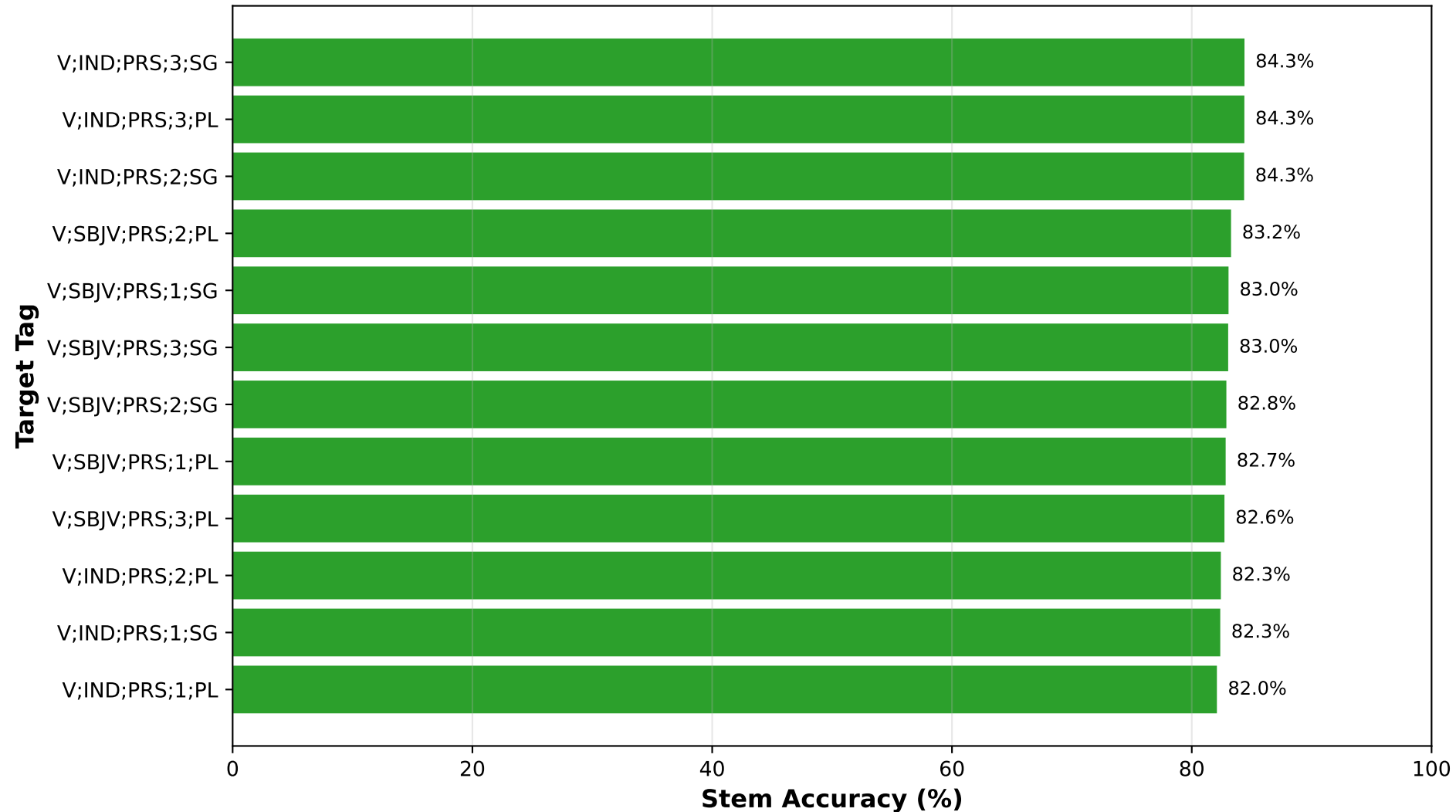
Stem Accuracy by Target Tag - 90%L-10%NL - Vanilla
