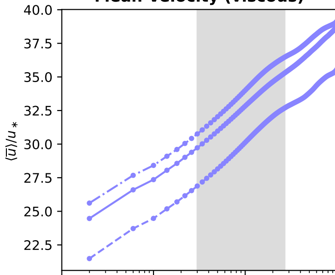
Mean Velocity (viscous)
