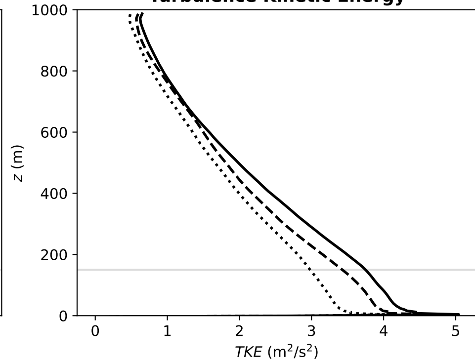
Turbulence Kinetic Energy
