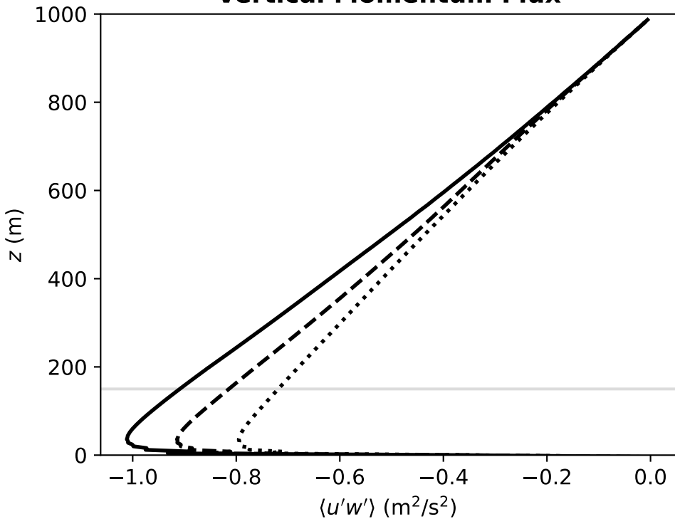
Vertical Momentum Flux
