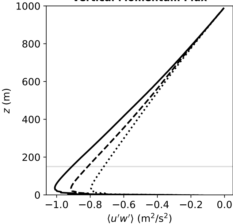
Vertical Momentum Flux
