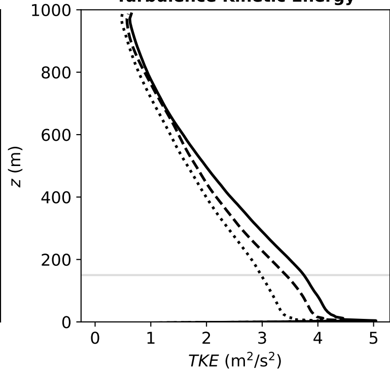
Turbulence Kinetic Energy
