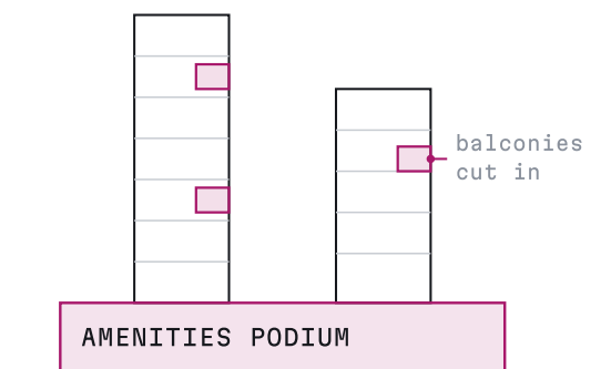
FIG 7.4 · Two towers of different height over one shared amenities podium, with the balconies cut into the facade rather than hung off it
