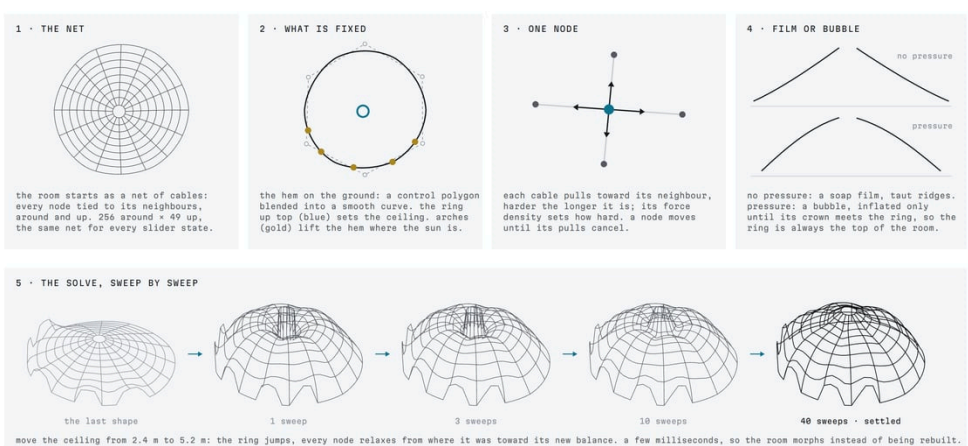
FIG 3.3 · How the room finds its shape: the net, what is fixed, one node's pulls cancelling, and the solve relaxing sweep by sweep
