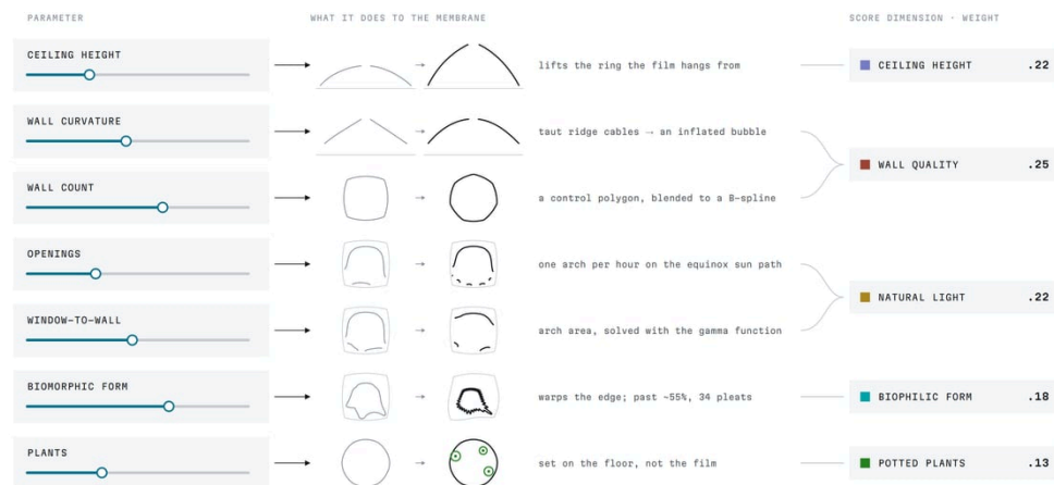
FIG 3.2 · The rules, drawn by the app's own solver: each slider, what it does to the membrane, and the score dimension it feeds
