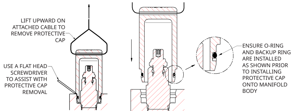
Figure 10. System Bypass and Relief Valve Protection Cap Removal and Installation
