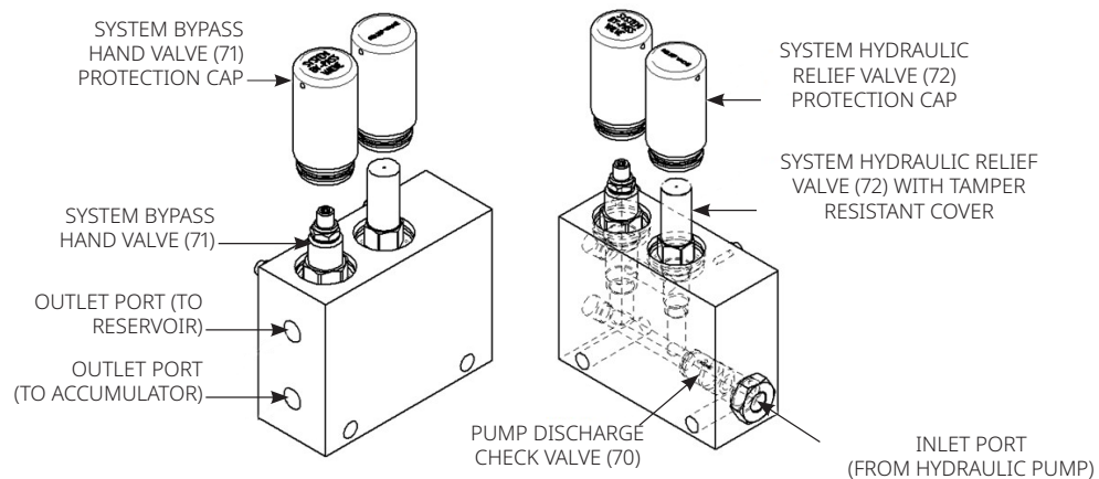
Figure 9. System Bypass and Relief Valve Diagram
