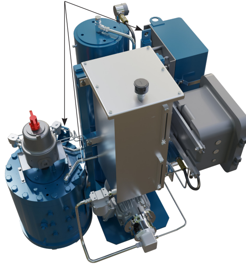
Figure 2. ECAT System Mounted on the Shafer Rotary Vane Actuator
