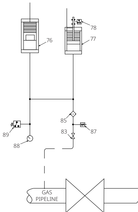
Figure 4. Typical ECAT Accumulator System (1)
