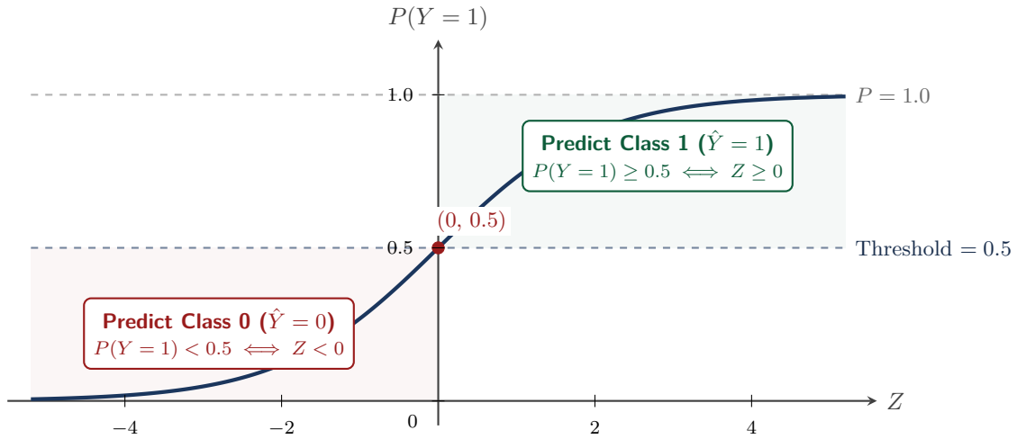
Figure 4.1: The Sigmoid activation function squashing unbounded linear values Z into valid class probabilities [0, 1] with a decision boundary at Z = 0 ( P = 0.5 ).
