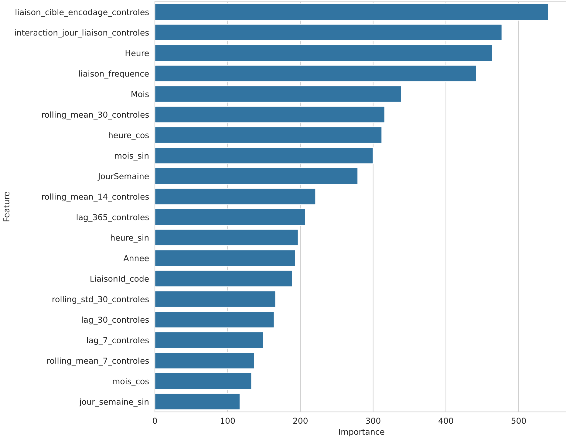
Importance des variables - LightGBM - J+7
