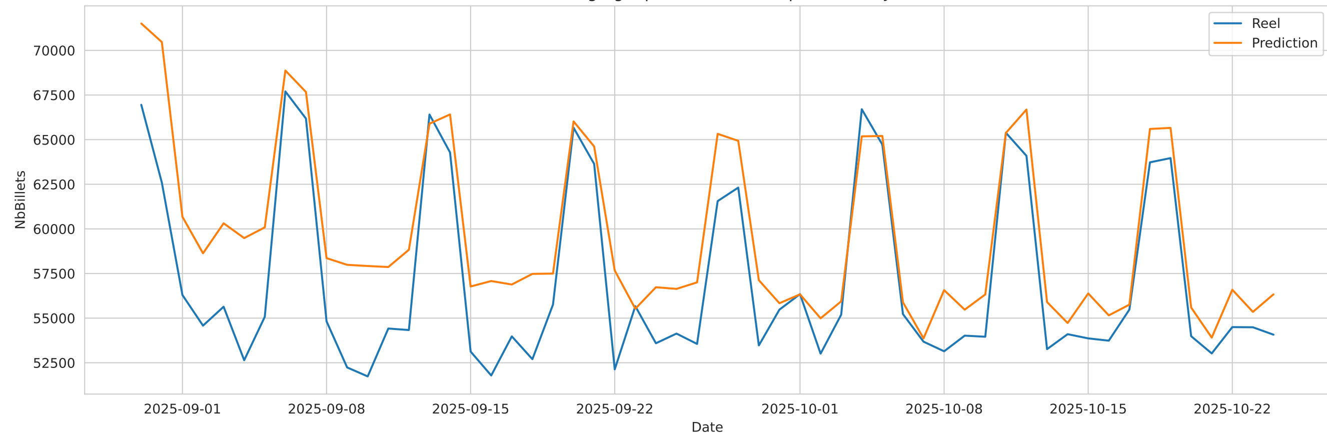
NbBillets agrege quotidien - reel vs prediction - J+7
