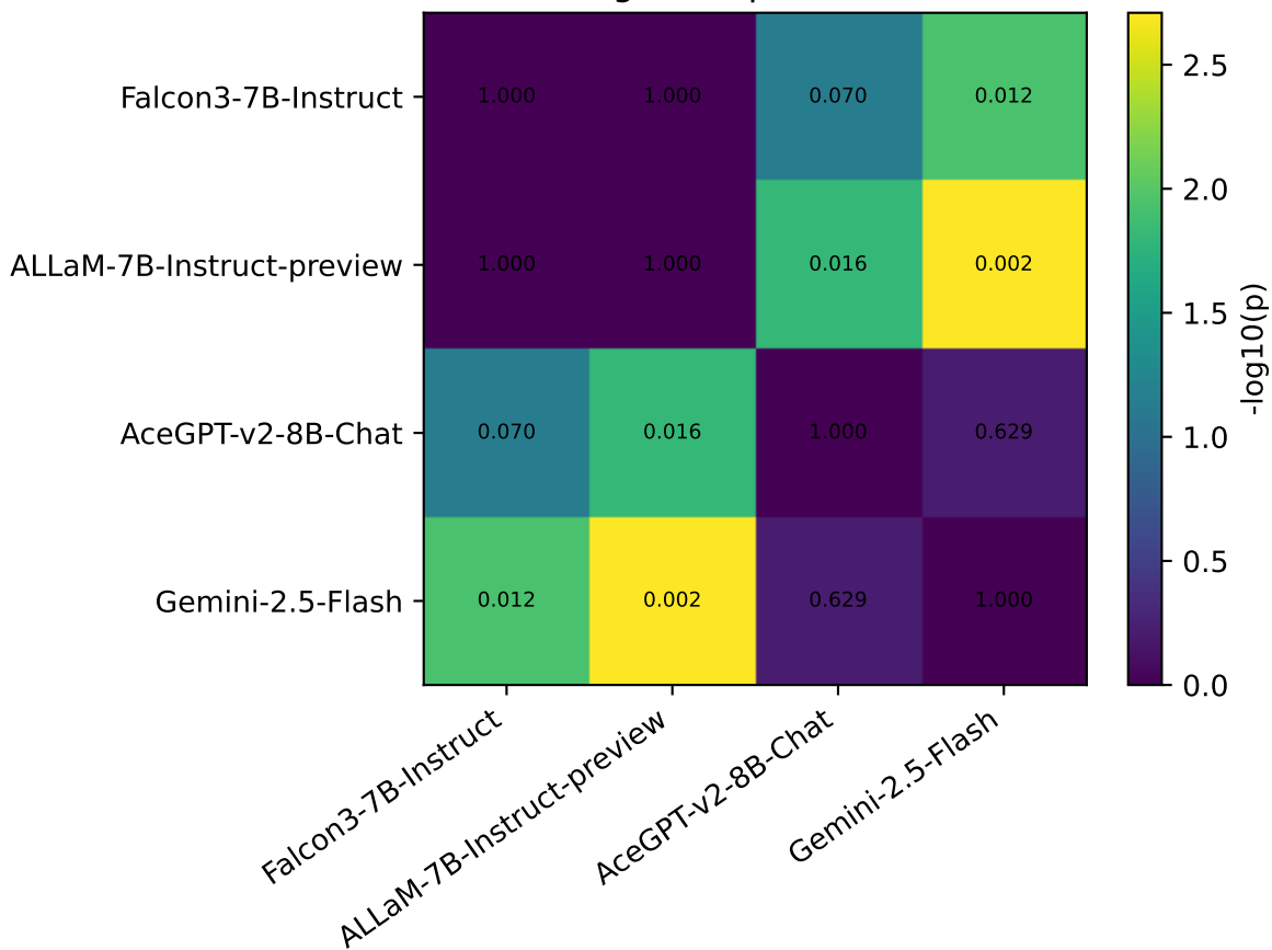
Paired sign-test p-values (Arabic)
