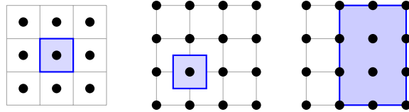
(a) Cell-centred (b) Vertex-centred (c) Cell-vertex
