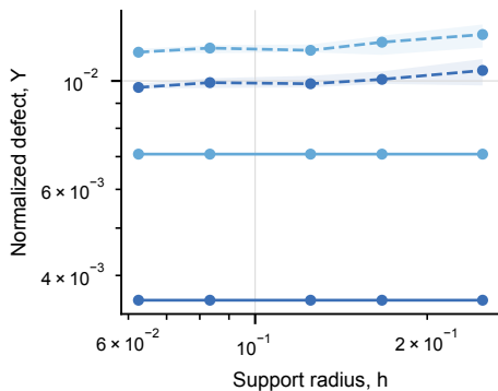
d Viscosity/Laplacian regular PASS; jitter FAIL
