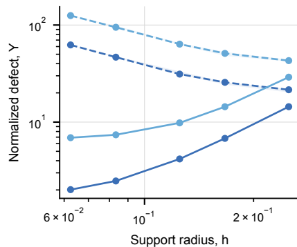
c Pressure gradient regular PASS; jitter FAIL
