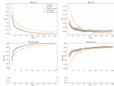
Activation Function Experiment Results (20 Epochs)
