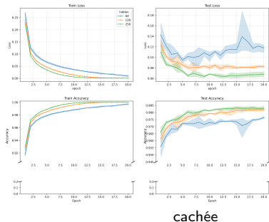
Hidden Size Experiment Results (20 Epochs)
