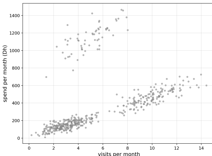
Figure 2.2: A store’s loyalty-card customers: monthly visits against monthly spend, as the file presents them, with no labels. Three groups of different sizes are plainly visible, and each one, taken alone, looks like a Gaussian cluster.
