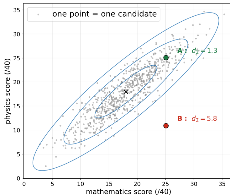
Figure 1.5: Two candidates at equal Euclidean distance from the mean candidate \boldsymbol{\mu} : the covariance structure makes A (strong in both papers) typical, d_\Sigma \approx 1.3 , and B (excellent in mathematics, poor in physics) an extreme anomaly, d_\Sigma \approx 5.8 .
