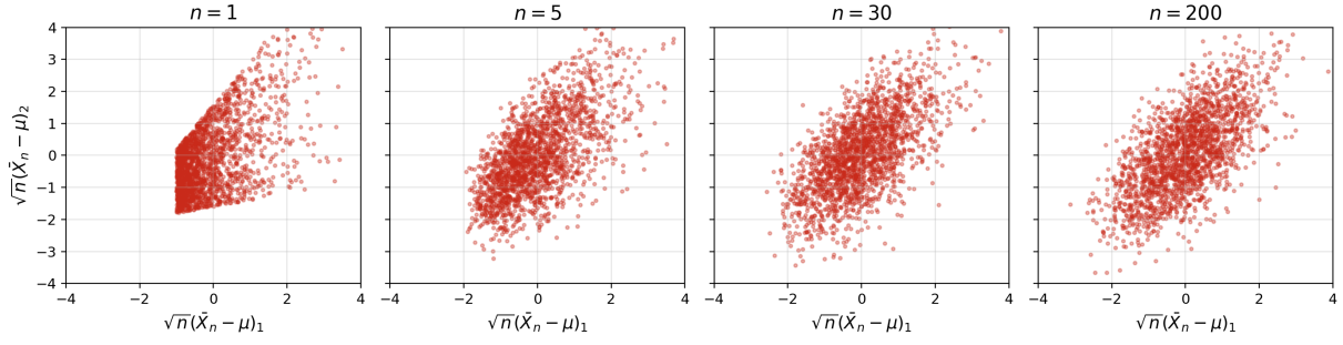
Figure 1.7: Rescaled means \sqrt{n}(\bar{\mathbf{X}}_n - \boldsymbol{\mu}) of a skewed 2D distribution with correlated coordinates: an elliptical Gaussian cloud, tilted by that correlation, emerges as n grows.
