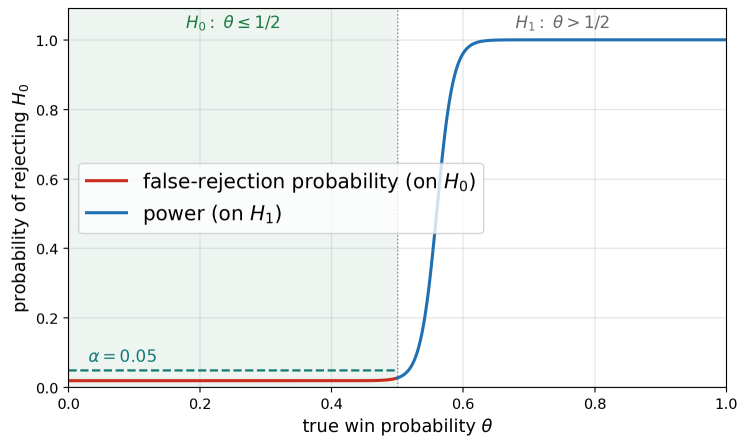
Figure 3.3: A rejection curve one would wish for, on the same axes: below the \alpha line throughout the null region, close to one throughout most of the alternative. At fixed n the rejection probability is continuous in \theta , so the steep rise can never be a jump; larger n steepens it.
