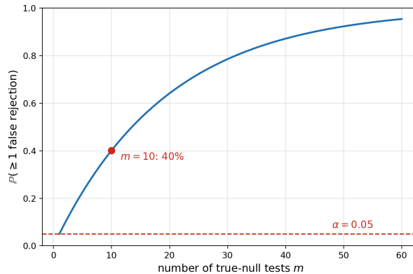
Figure 3.6: The probability (37) of at least one false rejection among m independent true-null tests at \alpha = 5\% : 40% at m = 10 , near certainty long before m = 200 .
