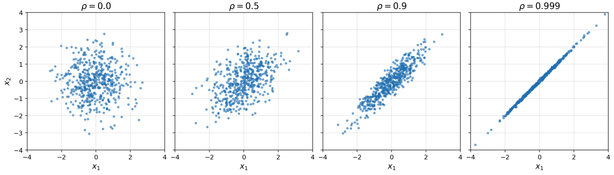
Figure 1.2: Samples of \mathcal{N}(0, \Sigma) with unit variances and correlation \rho : the cloud flattens onto a line as \rho \rightarrow 1 .
