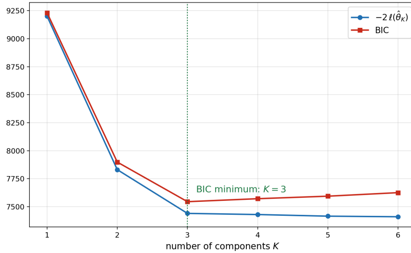
Figure 2.5: Model selection on the customers cloud (three latent groups). The fit term -2\ell(\hat{\theta}_K) decreases forever; BIC adds the penalty p_K \log n (the widening gap) and turns into a minimum at K = 3 .
