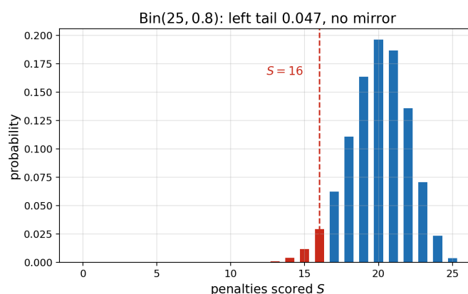
Figure 3.5: The penalty null \text{Bin}(25, 0.8) is skewed: the observed left tail (0.047) has no mirror image, and the two-sided p-value depends on a convention.
