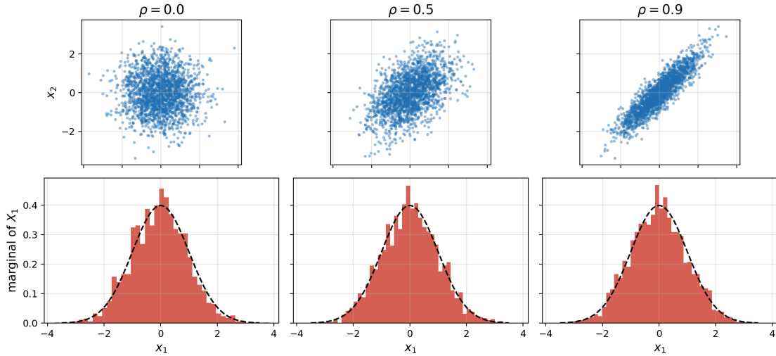
Figure 1.3: Correlated Gaussian samples (top row) and the marginal distribution of X_1 (bottom row): Gaussian at every correlation level.
