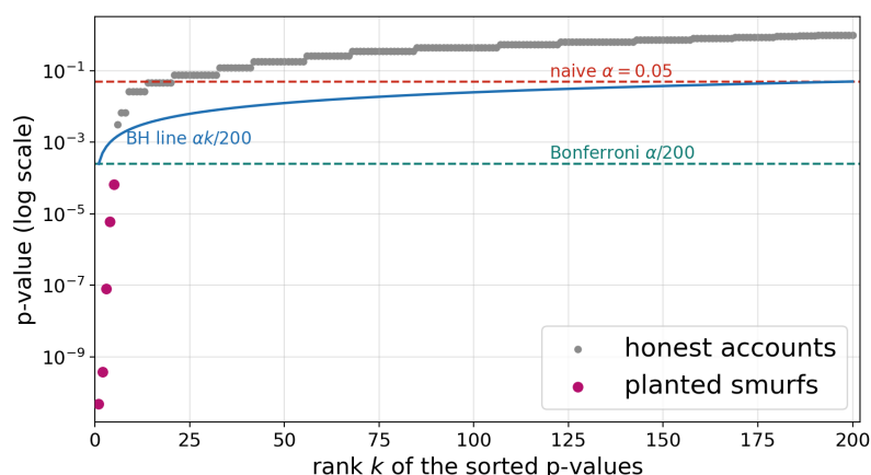
Figure 3.7: The 200 sorted p-values of the smurf screen (log scale). The five planted smurfs sit far below the Bonferroni threshold \alpha/200 ; fifteen honest accounts fall between the BH line and the naive 5% line and are flagged only by the naive screen. The staircase pattern in the honest p-values is the discreteness of section 3.2.4 again: with 60 games, only 61 p-values are possible.
