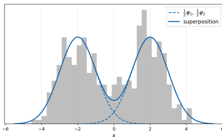
Figure 2.1: A sample with two equal groups (gray histogram), the two half-weighted Gaussian densities (dashed), and their superposition (solid): a two-peaked density that no single Gaussian can produce.
