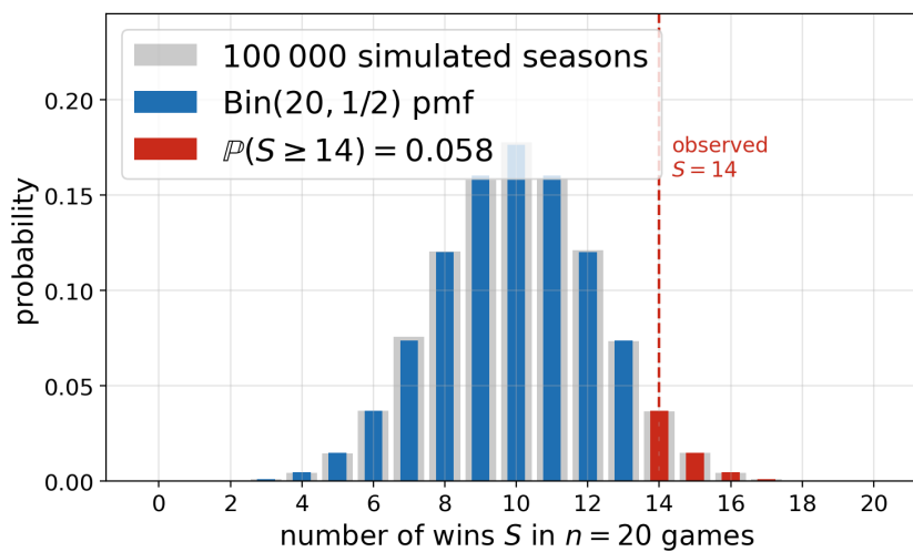
Figure 3.1: The null distribution of the number of wins S in 20 games: the exact \text{Bin}(20, 1/2) probabilities (blue) and the histogram of 100 000 simulated fair seasons (gray) agree. The observed S = 14 sits in the right tail; the red bars are the outcomes at least as favorable to Karim, of total probability 0.058.
