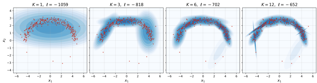
Figure 2.4: Fitted mixture density (blue, log scale) on a crescent-shaped cloud for a growing number of components. The log-likelihood increases at every step. At K = 12 several components have contracted onto a few points (the needle-thin ridges), and further gains come from sharpening these spikes, not from fitting the shape of the cloud: the onset of component collapse.
