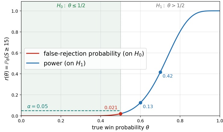
Figure 3.2: The rejection probability r(\theta) = \mathbb{P}_\theta(S \geq 15) of the rule “reject when S \geq 15 ” ( n = 20 ), over the whole parameter range. Over the shaded null region its height is a false-rejection probability, largest at the boundary: r(1/2) = 0.021 , below the \alpha line. Over the alternative region the same height is the power: 0.13 at \theta = 0.6 , 0.42 at 0.7.
