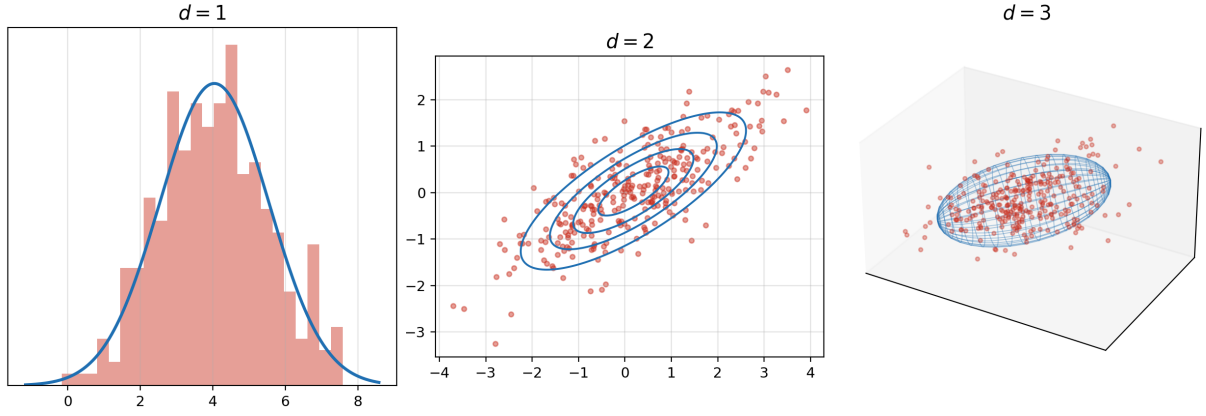
Figure 1.9: One Gaussian cluster in d = 1, 2, 3 : data (red) and the fitted Gaussian (blue). In every dimension the fitted density is characterized by its mean and covariance alone: mass symmetric around the mean, level sets ellipsoids whose orientation and elongations the covariance defines.
