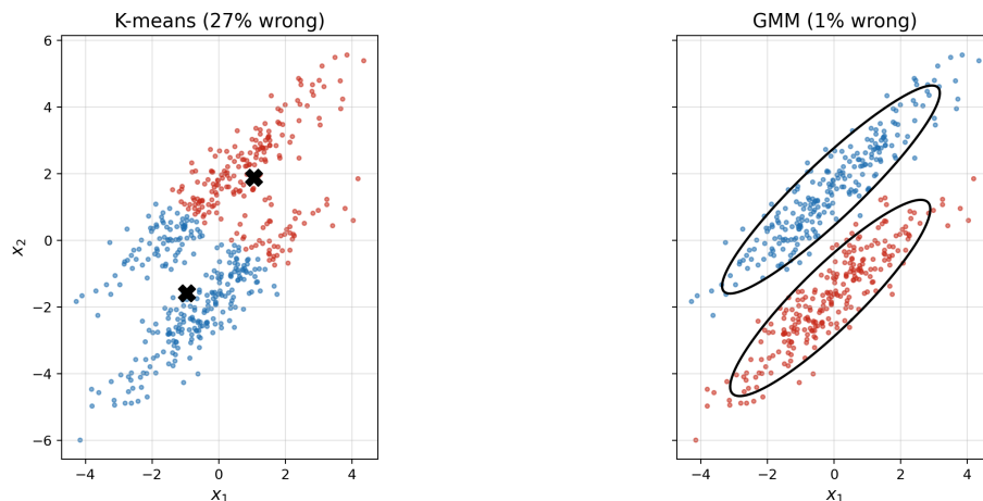
Figure 2.6: Two elongated correlated clusters. K-means (left) assumes spherical clusters and slices across the true groups; the full-covariance GMM (right) models the shape and recovers them.
