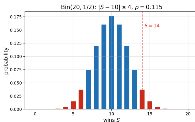
Figure 3.4: Under the symmetric null \text{Bin}(20, 1/2) , the two-sided region |S - 10| \geq 4 has two mirror-image tails, and the two-sided p-value doubles the one-sided one.
