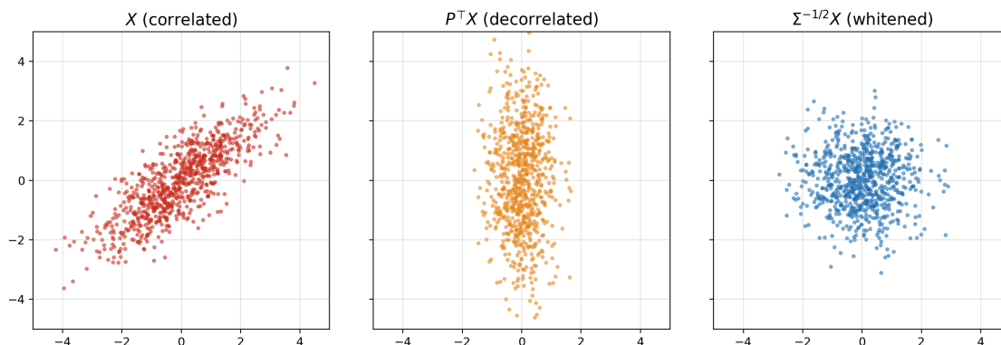
Figure 1.4: Whitening step by step: original, decorrelated ( P^\top(\mathbf{X} - \boldsymbol{\mu}) ), and whitened ( \Lambda^{-1/2}P^\top(\mathbf{X} - \boldsymbol{\mu}) , which equals \Sigma^{-1/2}(\mathbf{X} - \boldsymbol{\mu}) up to the rotation P ) samples.
