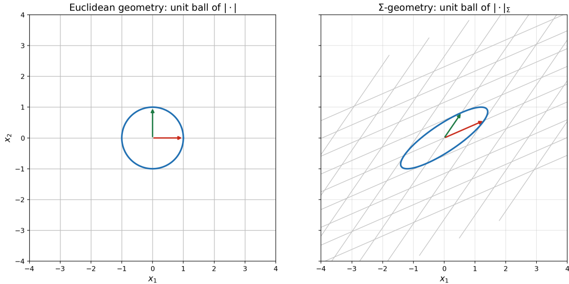
Figure 1.6: The scalar product \langle \mathbf{u}, \mathbf{v} \rangle_{\Sigma} = \mathbf{u}^{\top} \Sigma^{-1} \mathbf{v} replaces the Euclidean geometry (left: square grid, unit circle) by an anisotropic one (right: the square grid mapped by \Sigma^{1/2} , an oblique lattice; the unit ball is the covariance ellipse). The arrows are the images of the standard basis: unit vectors of the new geometry.
