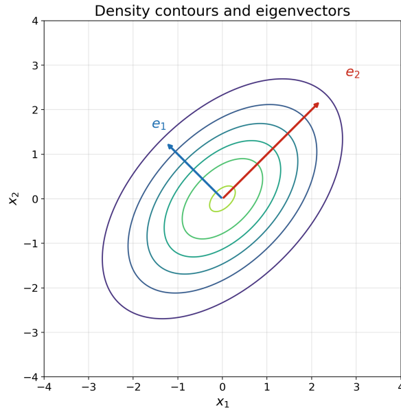
Figure 1.1: Density contours of \mathcal{N}(0, \Sigma) , with the eigenvectors of \Sigma (here \Sigma_{11} = \Sigma_{22} = 2 , \Sigma_{12} = 1 ). The long axis follows the top eigenvector of \Sigma .
