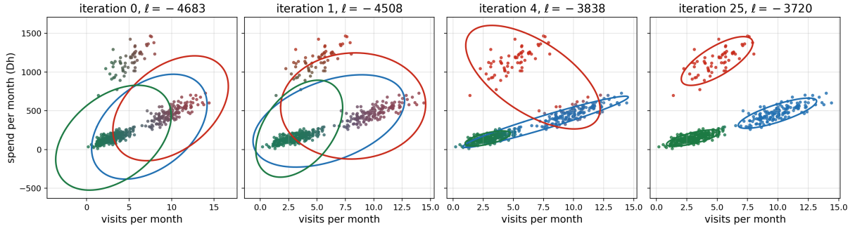
Figure 2.3: One EM run ( K = 3 ) on the customers cloud: point colors blend the component colors in proportion to responsibilities; ellipses are the current component covariances. The log-likelihood increases at every step, as theorem 2.3.1 promises for the exact M-step (the run adds the tiny ridge of section 2.4).
