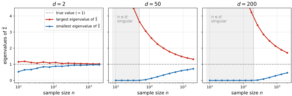
Figure 1.8: Largest and smallest eigenvalues of \hat{\Sigma}_{\text{MLE}} (averaged over 20 replications) as the sample size grows, on data from \mathcal{N}(0, \mathbf{I}_d) where every true eigenvalue is 1. Left to right: d = 2, 50, 200 . In the shaded region n \leq d the smallest eigenvalue is exactly 0 (proposition 1.6.1); beyond it, convergence toward the truth is slower the larger d .
