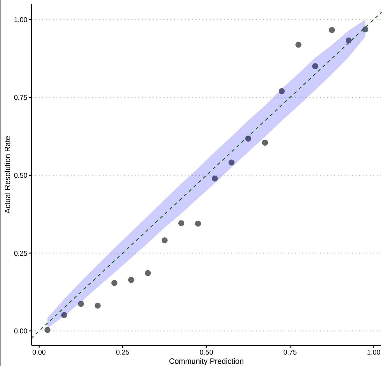
Metaculus Community Calibration (2022–2023, time-weighted)
