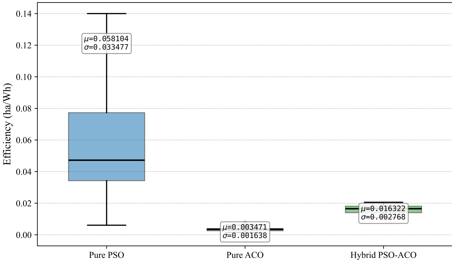
Area Coverage per Unit Energy
