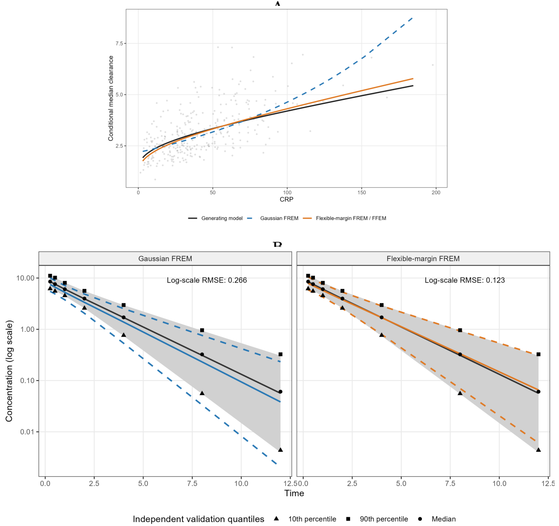
Figure 1: Conditional translation and prediction in the CRP example. (A) Exact FFEM/conditional median relationship; grey points are latent simulated clearances. (B) Conditional VPC above the 95th CRP percentile. Grey and black show the generating distribution; coloured lines show fitted quantiles and black points independent validation quantiles. Albumin was integrated out. Flexible margins reduced log-scale VPC RMSE from 0.266 to 0.123.
