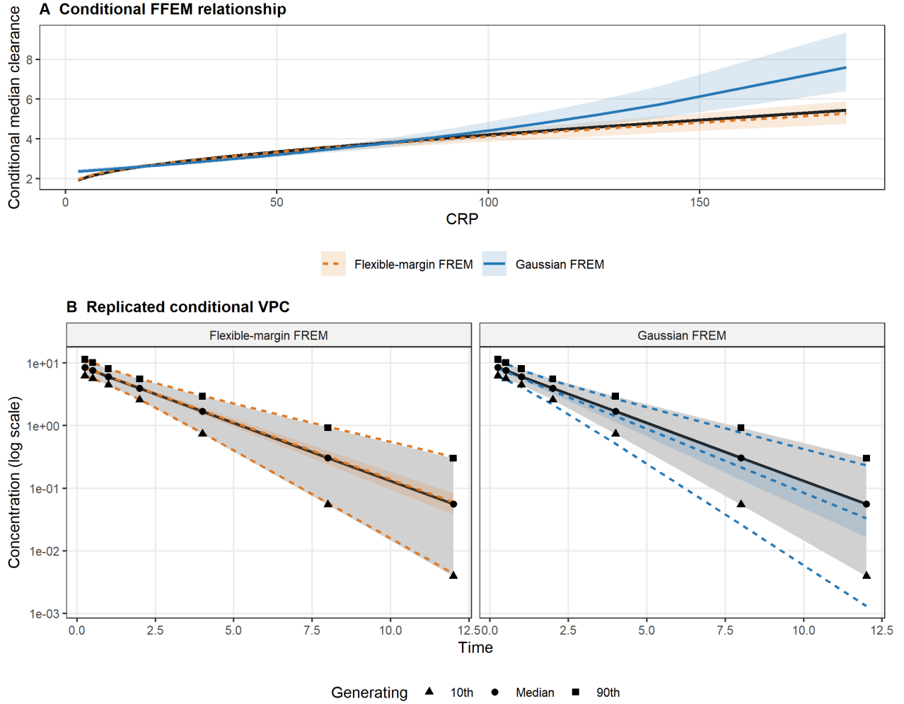
Figure 2: Conditional results across 200 independently fitted datasets. (A) Median FFEM/conditional relationships; ribbons are pointwise 2.5th–97.5th percentiles across fits and the black line is the generating relationship. (B) Replicated conditional VPC. Grey regions and black symbols show the generating 10th (triangle), 50th (circle) and 90th (square) percentiles. Coloured dashed lines are median fitted quantiles across the 200 fits; coloured ribbons are pointwise 2.5th–97.5th percentiles for the fitted median.
