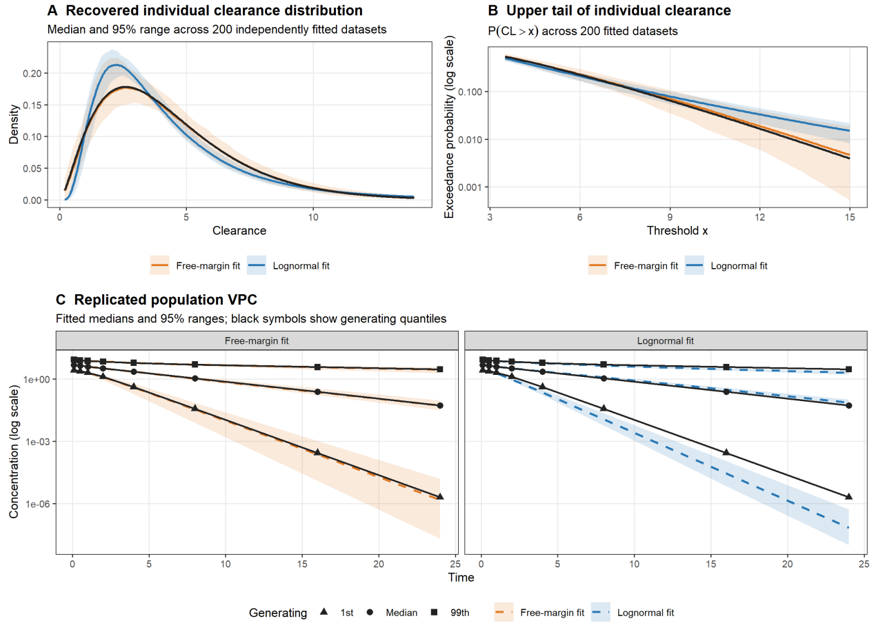
Figure 1: Natural-parameter marginal validation across 200 independent datasets. (A) Generating Gamma clearance density (black) and median fitted densities with pointwise 95% ranges. (B) Corresponding upper-tail probabilities. (C) Replicated population VPC for automatically selected free margins and standard lognormal clearance. Black symbols denote generating 1st (triangle), 50th (circle) and 99th (square) percentiles; coloured dashed lines and ribbons are fitted medians and pointwise 95% ranges.
