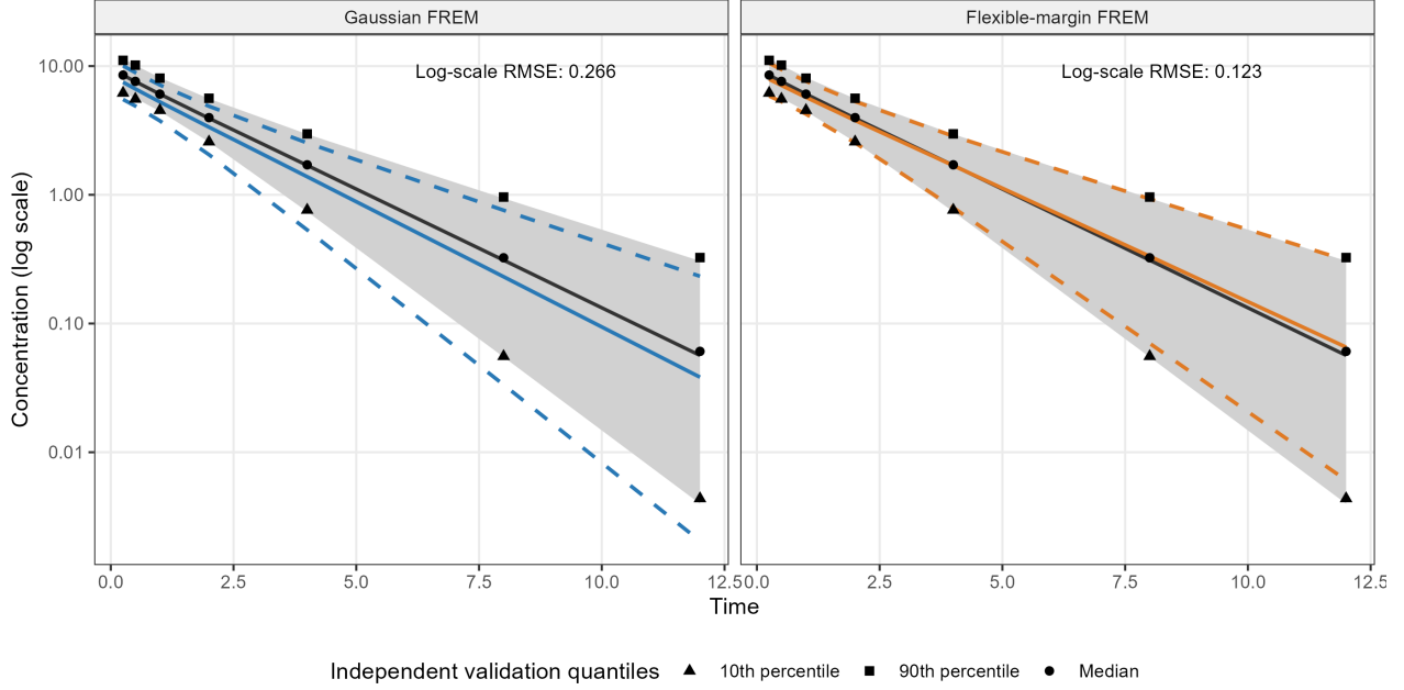
Figure 1: Conditional VPC in an independent population above the 95th CRP percentile. Grey shading and the black line show the generating 10th–90th percentile interval and median. Coloured solid and dashed lines show fitted median and 10th/90th percentiles; black points show empirical quantiles in the independent validation sample. Only CRP was available for prediction; albumin was integrated out. Flexible-margin FREM reduced log-scale VPC RMSE from 0.266 to 0.123.
