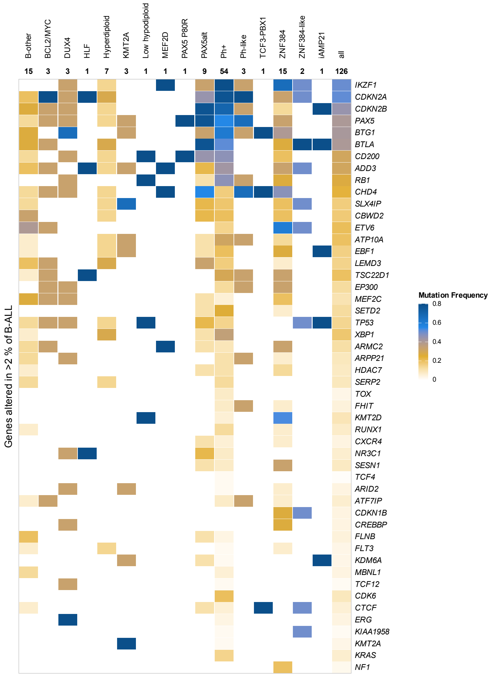
Mutation Frequency per subtype
