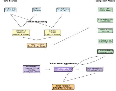
Figure 1: Super Ensemble Architecture Flowchart. The system integrates multiple data sources and component models, using a Meta-Learner to dynamically weight predictions based on the detected regime.
