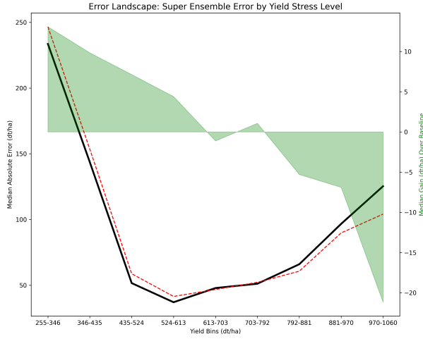
Figure 3: Super Ensemble error landscape across yield stress levels. The ensemble achieves its largest gains over the baseline in extreme low-yield regimes (255–613 dt/ha), where errors are reduced by up to \sim 10 dt/ha. Performance is the same in the mid-range (613–792 dt/ha), while the ensemble underperforms the baseline at high yields (above 792 dt/ha).
