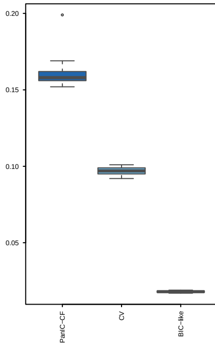
Logistic
