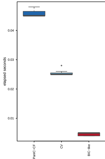
Gaussian
