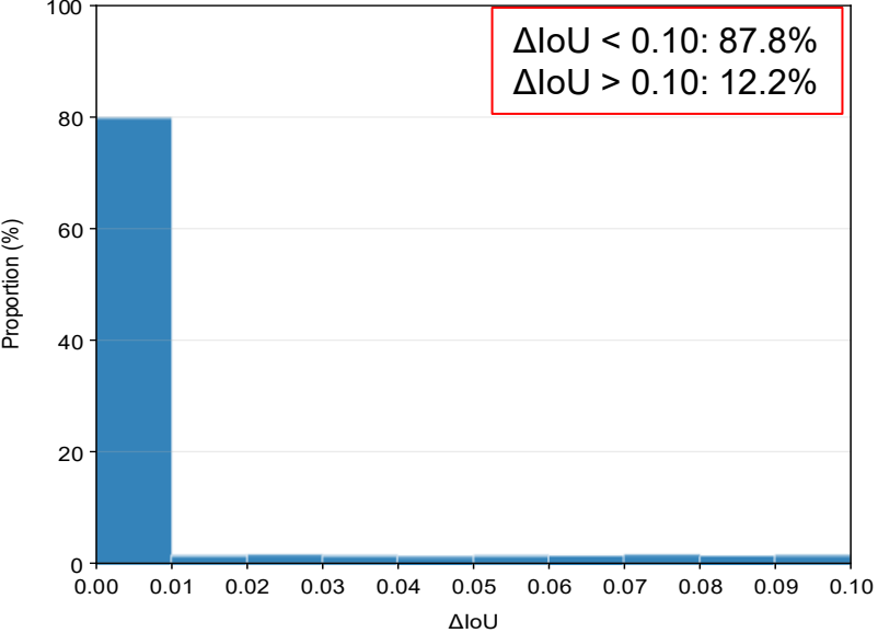
ActivityNet-Captions
