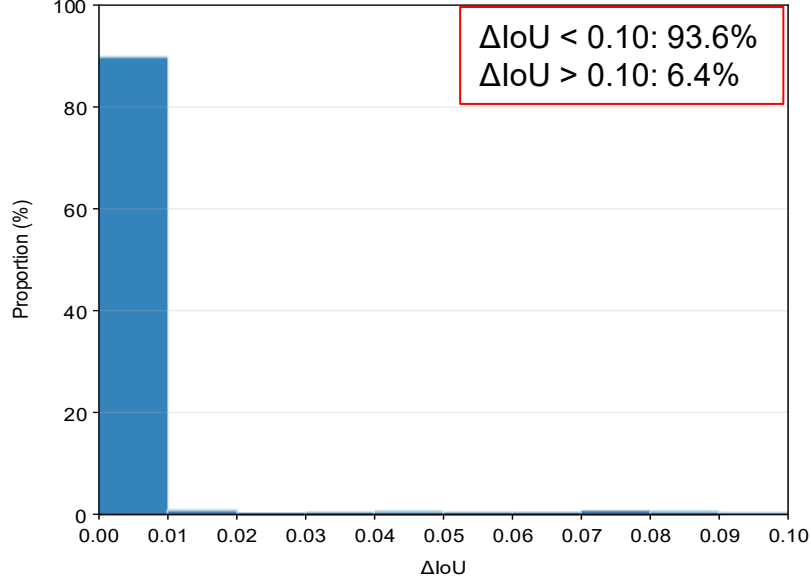
Charades-STA
