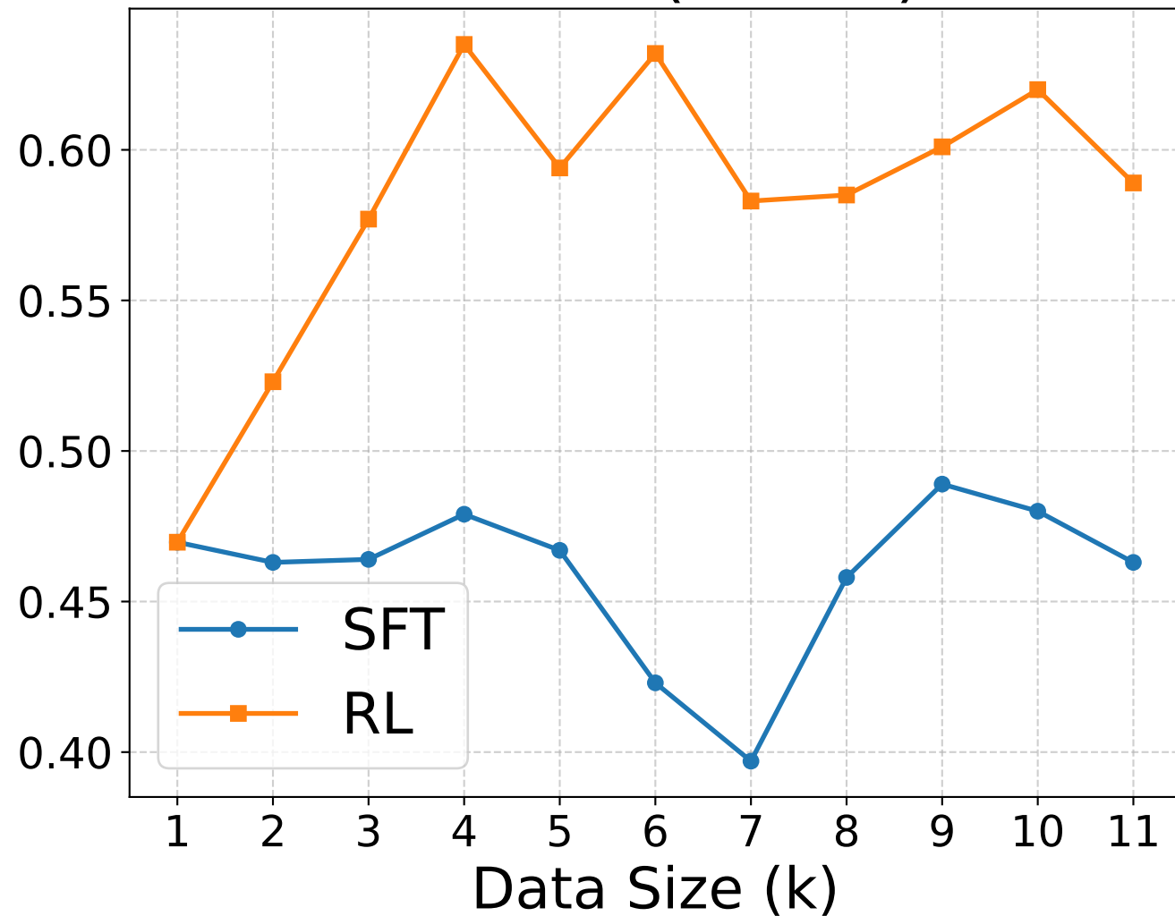
Formula(1-NED)
