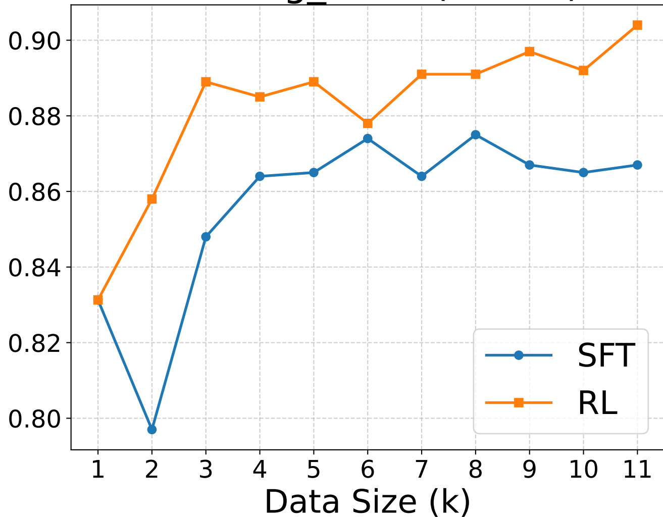
Reading_Order(1-NED)
