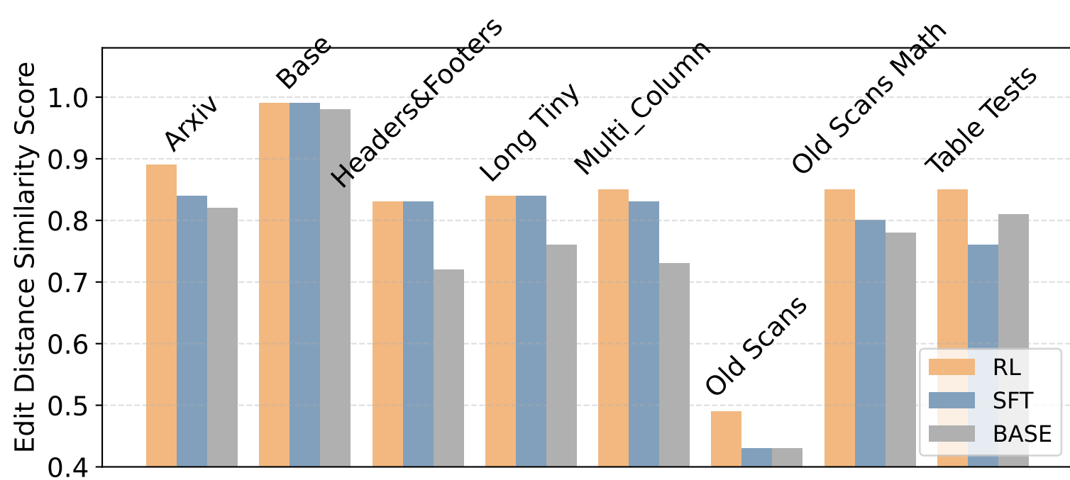
(a) olmOCR across multiple document domains
