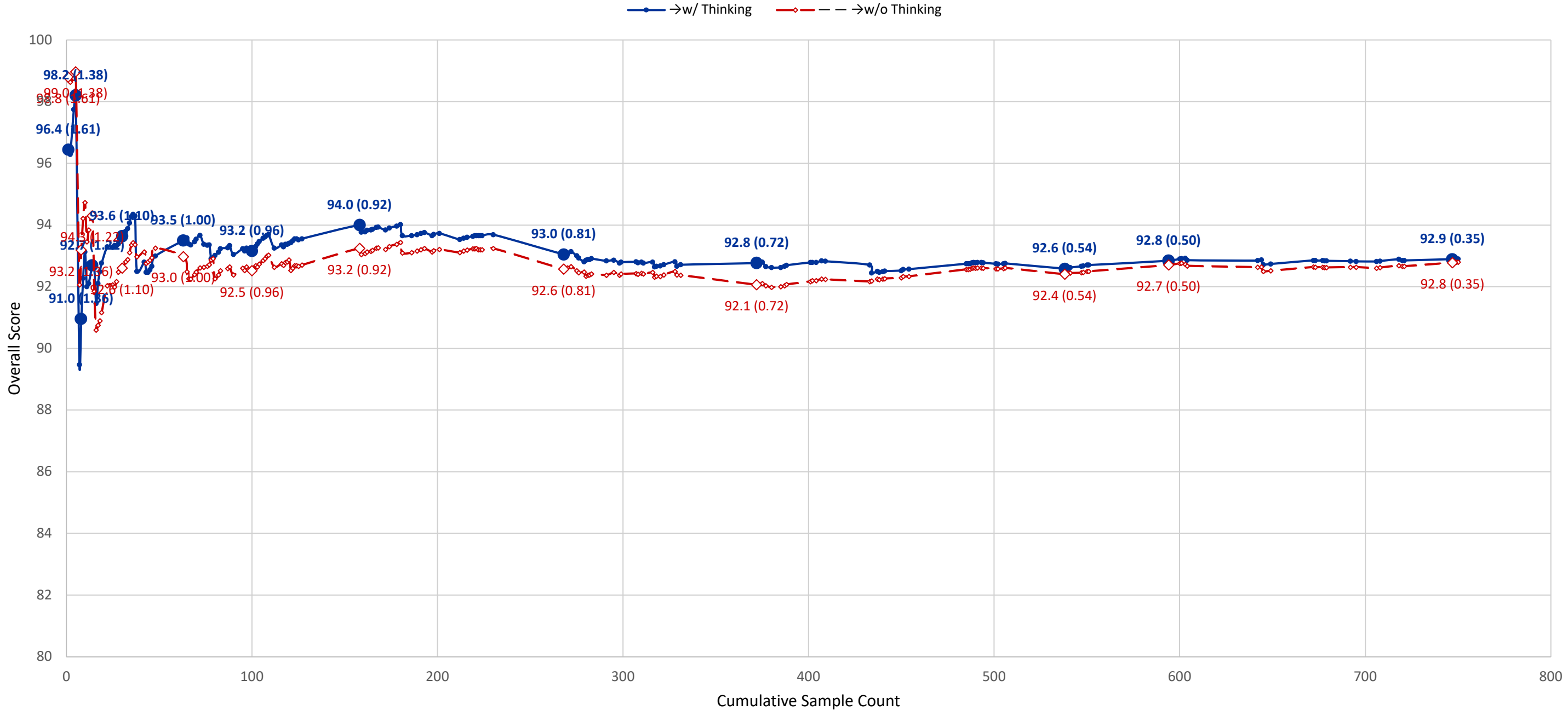
Overall Score on Omni-Doc-Bench-v1.5 by Cumulative Sample Count (Samples Sorted by Layout Label Entropy in Descending Order)
