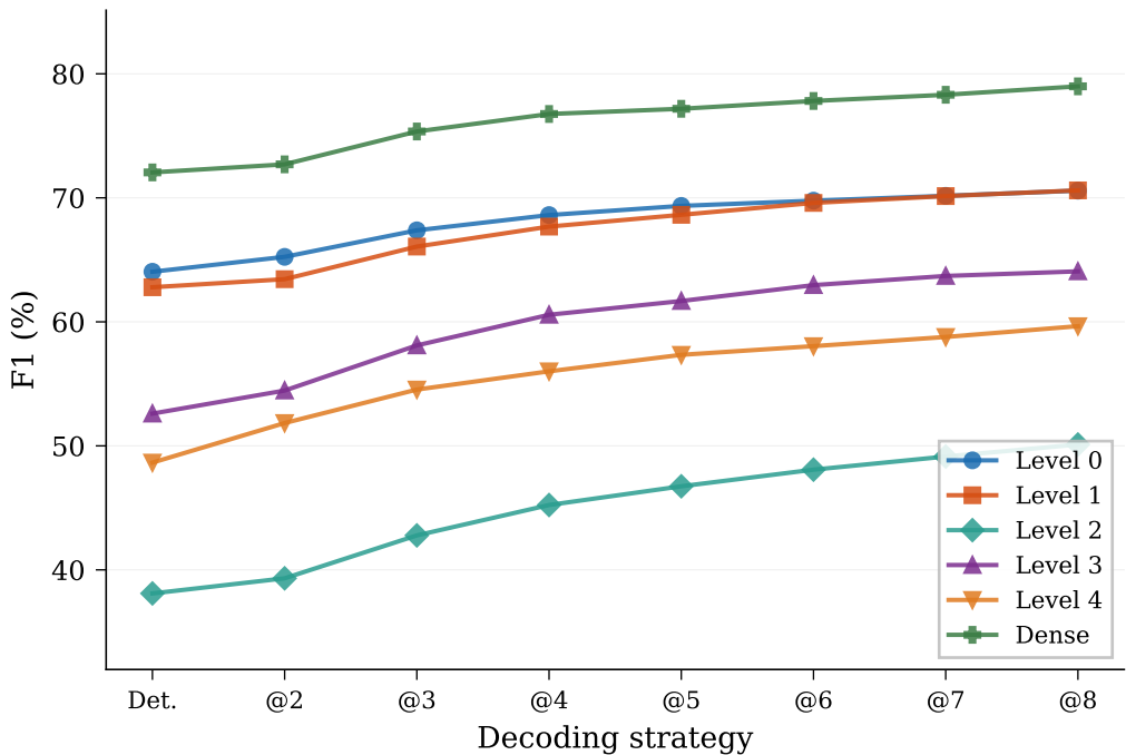
PBench — Deterministic vs Pass@k (k = 2 .. 8)
