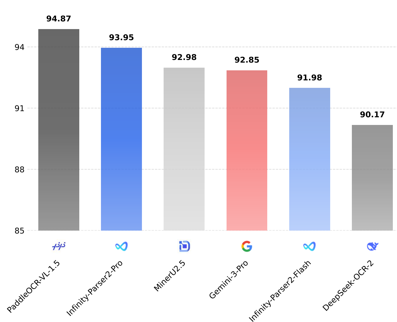
OmniDocBench-v1.6
