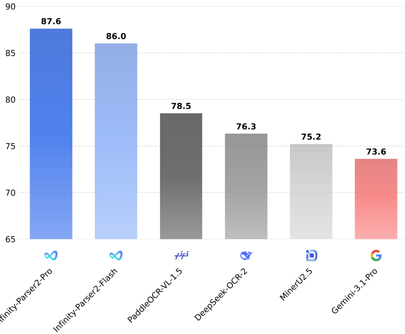
olmOCR-bench
