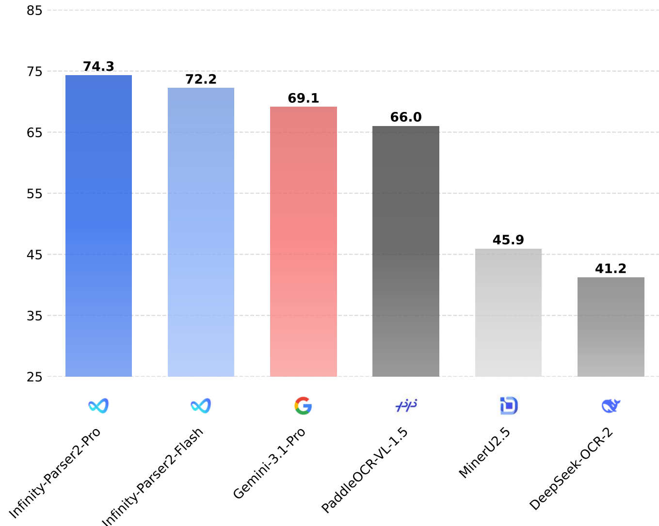
ParseBench
