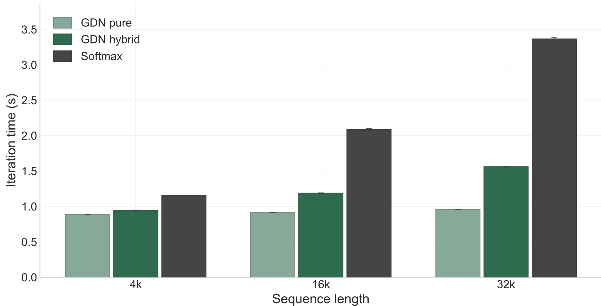
Iteration Time vs. Sequence Length
