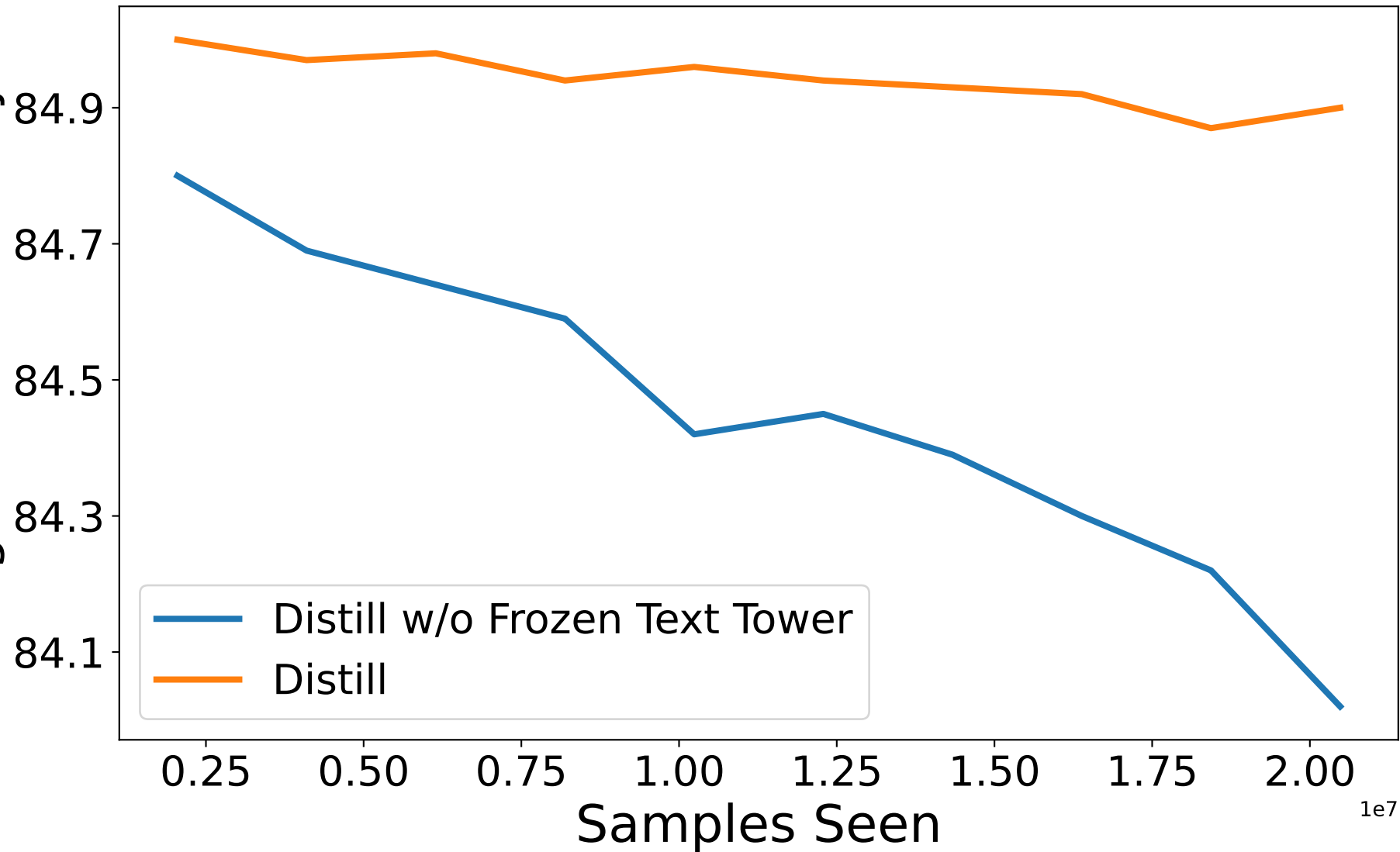
ImageNet 1K Accuracy
