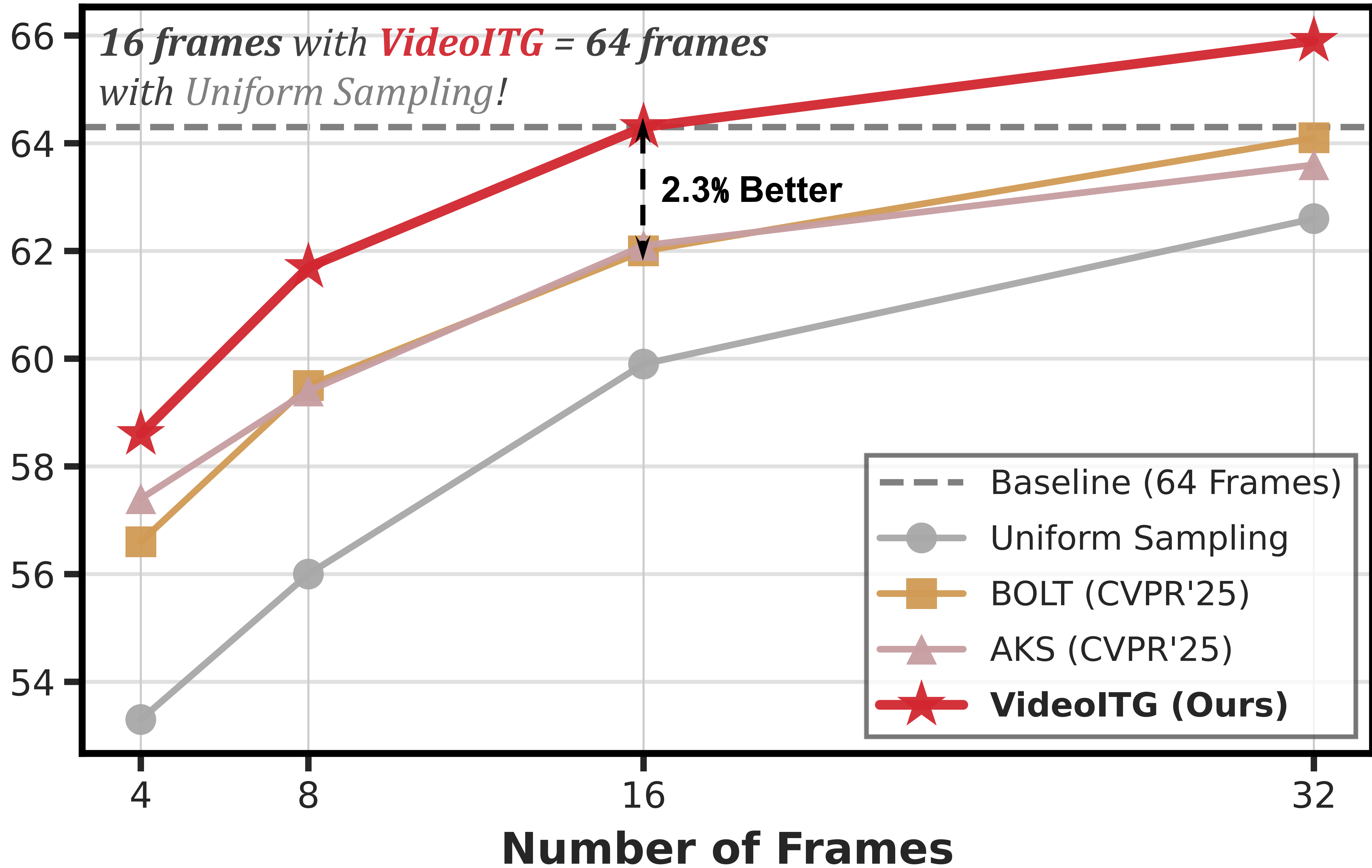
Performance on VideoMME
