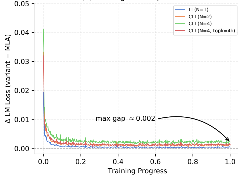
(a) Training Loss Gap vs. MLA
