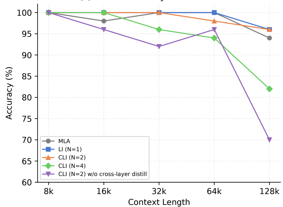
(c) Needle-in-a-Haystack Evaluation
