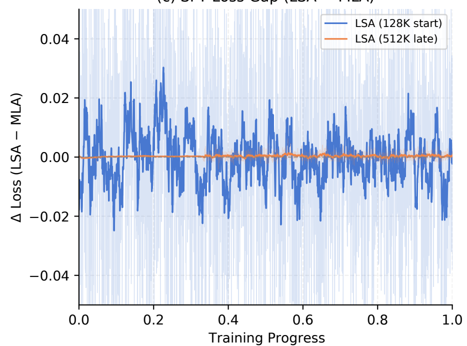
(c) SFT Loss Gap (LSA - MLA)
