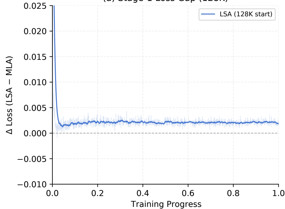
(a) Stage-1 Loss Gap (128K)
