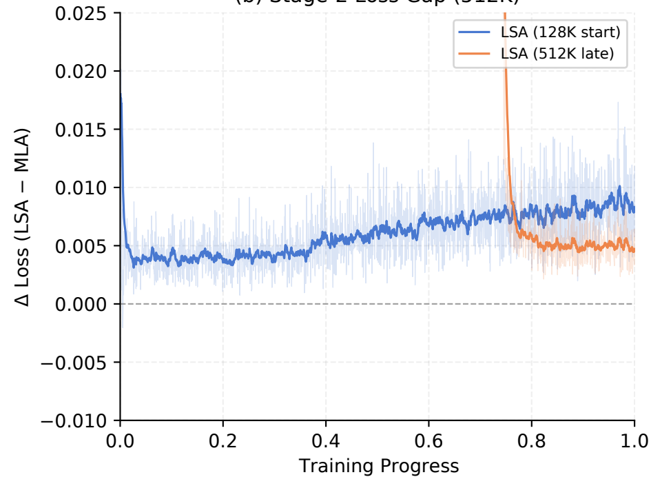
(b) Stage-2 Loss Gap (512K)
